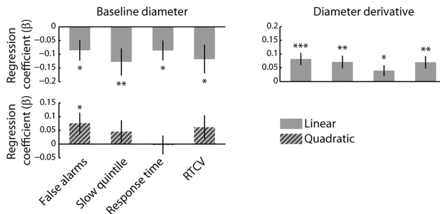
Fig 4. The relationship between pupil diameter and behavior. Regression coefficients are shown per pupil measure and behavioral measure. USD: Units standard deviation. Error bars represent the SEM. *: p < 0.05 ; **: p < 0.01 ; ***: p < 0.001 .
