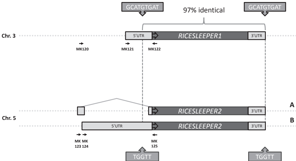
Figure 6. Comparison of the RICESLEEPER1 and 2 loci. Coding regions and part of the 5' and 3'UTR's are ~97% identical. RICESLEEPER1 and 2 each have obtained a new 5'UTR sequence, which is not homologous to that of the other locus. A and B display two different transcription models found by PCR for RICESLEEPER2 . Transcription model B has most likely acquired sequence material from a retrotransposon insertion in an intron on the opposite strand. Short duplications were found flanking the zones of homology in both genes, which are shown in arrowed boxes. The small arrows represent PCR primers, which were designed on available rice gene expression data, and were used to obtain RICESLEEPER1 and 2 transcripts from a cDNA library. Primer descriptions can be found in Table S2.
