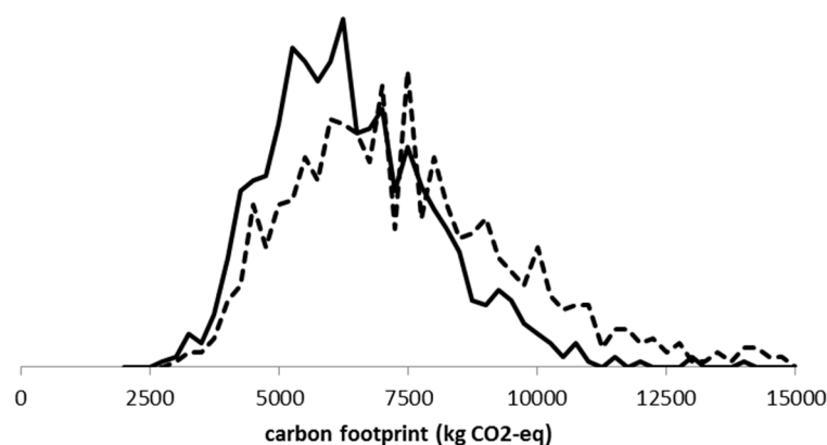
Figure 3. Probability density functions of the carbon footprint of a Vietnamese aquaculture system of Pangasius catfish, obtained from two artificial samples: large-scale (solid line) and small-scale (dashed line).
