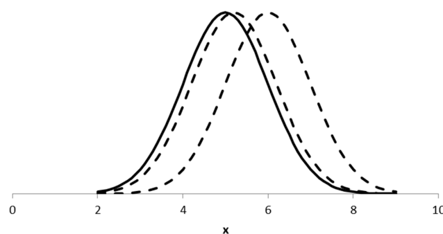
Figure 2. Probability density function for Y_A \sim N(5.0, 1) (solid line) and Y_B \sim N(5.2, 1) and Y_B \sim N(6.0, 1) (two dashed lines), corresponding to standardized effect sizes \delta = 0.2 (small) and 1.0 (large).
