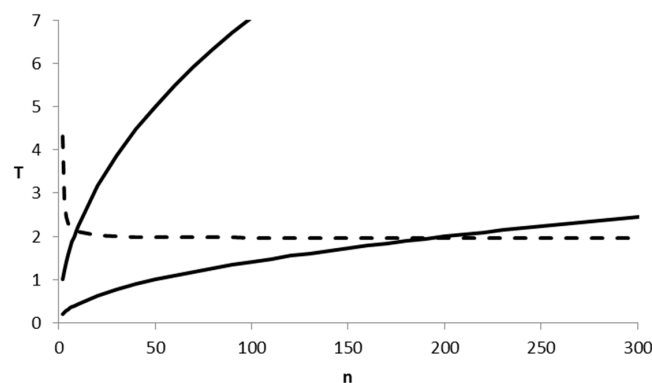
Figure 1. The absolute value of the T -statistic when \bar{Y}_A = 5.0 , \bar{Y}_B = 6.0 , S_P = 1 (upper solid line) for different values of the sample size n , when \bar{Y}_A = 5.0 , \bar{Y}_B = 5.2 , S_P = 1 top (lower solid line), and the upper critical value of the t -distribution (dashed line) at \alpha = 0.05 . The null hypothesis of equality of population means is rejected at 0.05 for n \geq 9 when \Delta\bar{Y} = 1.0 , but when \Delta\bar{Y} = 0.2 , we need to push further and use n \geq 194 to do the job.
