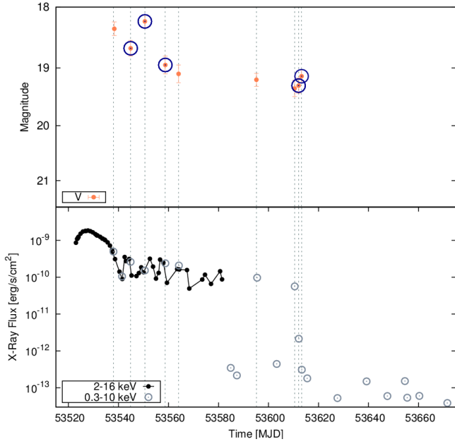
Figure 3. Top Panel: v band lightcurve (Swift/UVOT) of SAX J1808.4-3658 during the 2005 outburst reflare. The magnitudes are not dereddened. Bottom Panel: 2005 outburst X-ray lightcurve observed with RXTE/PCA (2-16 keV) and Swift/XRT (0.3-10 keV).
