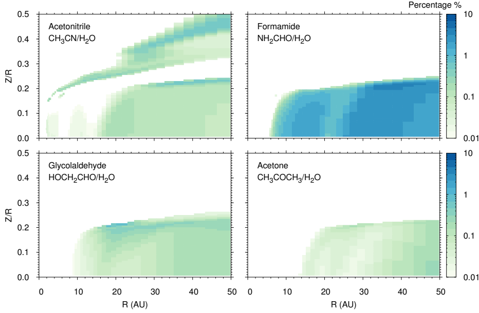
Fig. 2. Percentage of \text{CH}_3\text{CN} , \text{NH}_2\text{CHO} , \text{HOCH}_2\text{CHO} , and \text{CH}_3\text{COCH}_3 ice relative to water ice, as a function of disk radius, R , and height (scaled by the radius, Z/R ). Data are from Walsh et al. (2014).
