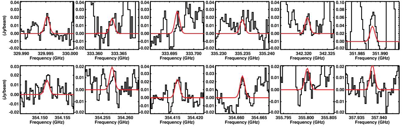
Fig. B.1. Black: Detected lines of NH 2 CDO. Red: Best-fit model for T_{\text{ex}}=300 K.
