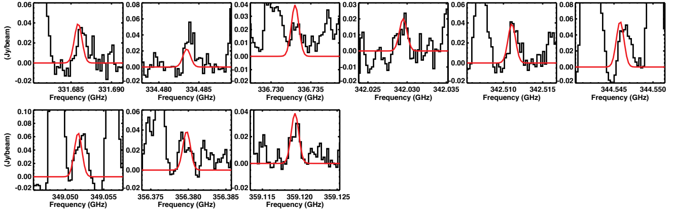
Fig. B.7. Black: Lines of \text{NH}_2\text{CHO } v=0 with the lowest opacities. Red: Model based on the analysis of the \text{NH}_2^{13}\text{CHO} lines and a ^{12}\text{C}/^{13}\text{C} ratio equal to 68.
