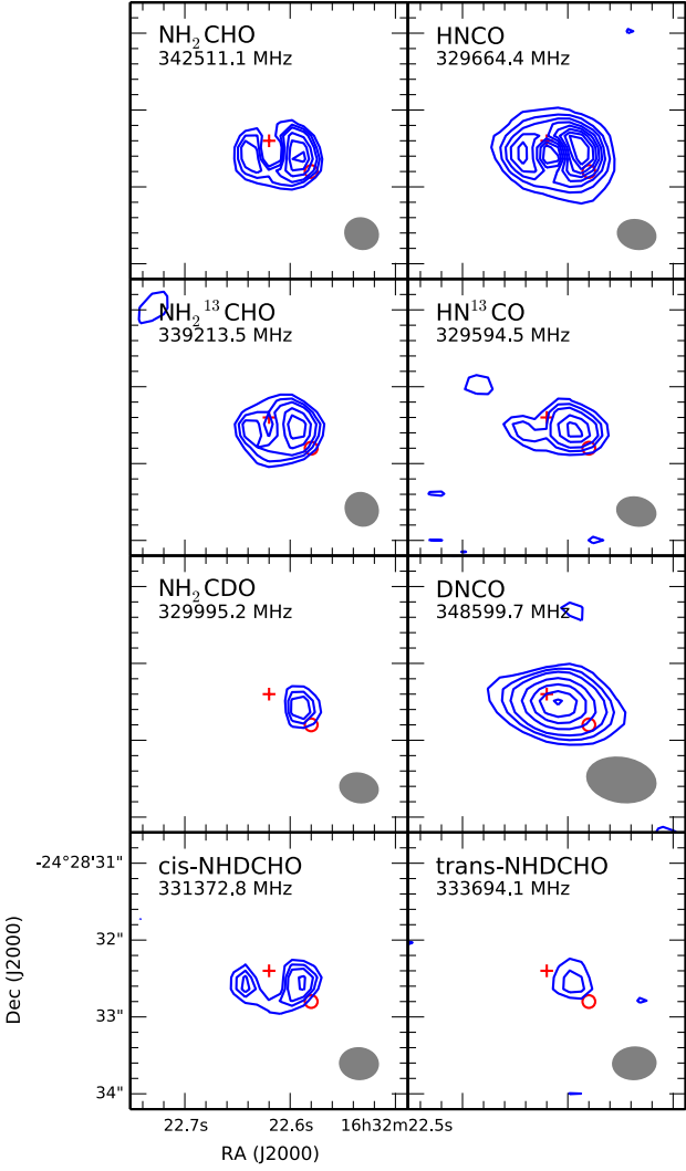
Fig. 1. Integrated intensity maps of \text{NH}_2\text{CHO} , \text{HNCO} and their isotopologues towards source B. The position of the continuum peak of source B is indicated with a red cross, while the position where the spectrum was extracted is shown with a red circle. The beam sizes are shown in grey in the bottom right corner of each panel. The contour levels start for the main isotopologue of \text{HNCO} at 0.05 \text{ Jy km s}^{-1} with a step of 0.05 \text{ Jy km s}^{-1} . For the other species, the levels are 0.02, 0.03, 0.04, 0.06, 0.08, 0.1 and 0.12 \text{ Jy km s}^{-1} .
