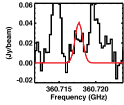
Fig. B.8. Black: Line of \text{NH}_2\text{CHO } v_{12}=1 with the lowest opacity. Red: Model based on the analysis of the \text{NH}_2^{13}\text{CHO} lines and a ^{12}\text{C}/^{13}\text{C} ratio equal to 68.
