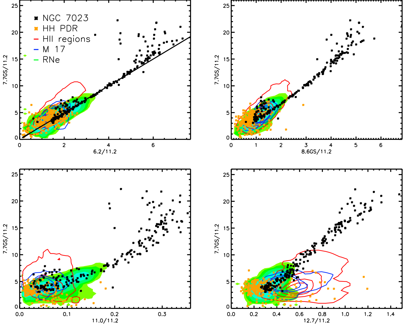
FIG. 5.— PAH band ratio correlations, where for each panel we have only included points where the S/N of our measurement of the ratio exceeds three. For the 6.2 vs. 7.7 correlation we have included a straight line generated by assuming a constant 6.2 vs. 7.7 band ratio and variable 11.2 band strength. Combined H II region points - red contours; NGC 1333 and 2023 - green to blue filled contours; NGC 7023 - black points; Horsehead - orange points; M17 - blue contour, contour levels given in Table 3.
