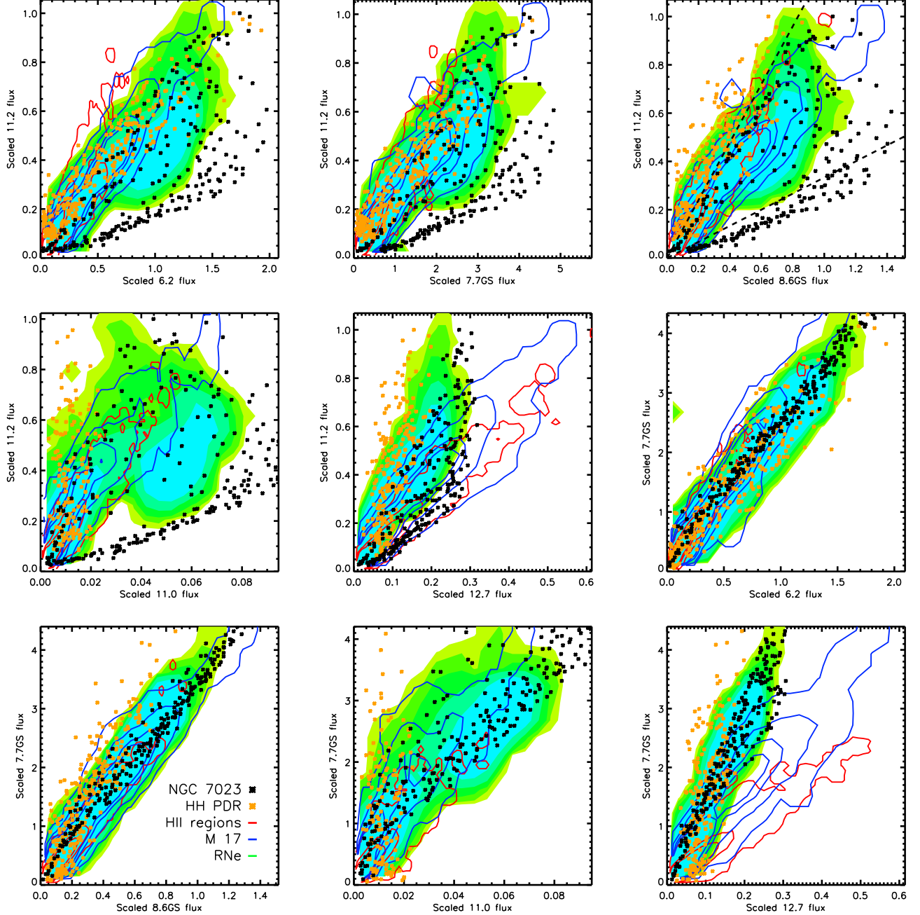
FIG. 7.— MIR emission component flux correlations with the 11.2\ \mu\text{m} PAH band (normalized to the peak 11.2 flux of each source). For each panel we have only included points for which there is a 3-sigma detection for each axis. In the rightmost panel of the top row we include the trends found by Boersma et al. (2014a) for the NGC 7023 data (see text) as dashed lines. Symbols and contours as in Figure 5, contour levels given in Table 3.
