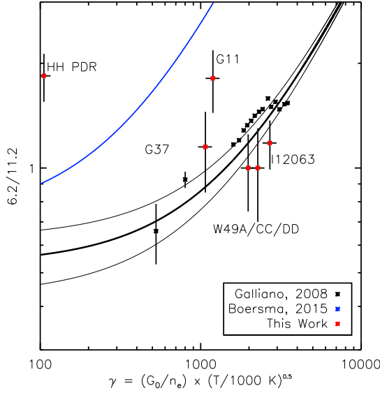
FIG. 9.— The empirical relationship between the PAH band intensity ratios and the physical conditions (collectively referred to as \gamma , see main text). The black points and line refer to the work of Galliano et al. (2008), where the thick line is the derived linear relationship between the black points and the thinner lines represent 1\sigma deviations. The red points represent the objects studied in this work, which seem to split into two groups, with four sources being consistent with the Galliano et al. (2008) line and two sources which are not.
