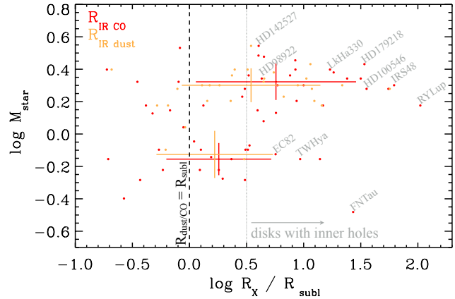
Figure 3. Measurements of R_{IR,dust} from IR interferometry (orange points, from Anthonioz et al. 2015; Menu et al. 2015) and of R_{IR,CO} from IR spectroscopy of CO gas (red points, from Banzatti & Pontoppidan 2015). The dust/CO radii ( R_x ) are normalized to the dust sublimation radii R_{subl} expected from models. Large crosses show median values and median absolute deviations for two stellar mass bins.
