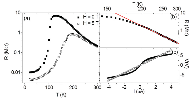
FIG. 2. (Color online) (a) R(T) behavior of a 5 \mu\text{m} \times 10 \text{ nm} LCMO bridge determined from I - V curves at an applied current of I = 0.1 \mu\text{A} at H = 0 \text{ T} (closed symbols) and H = 5 \text{ T} (open symbols) for the film on the unmilled STO substrate. (b) \log_{10} R vs T plot in the temperature range 150 – 300 \text{ K} for the same sample. Note: the scale on the T axis (top) is reciprocal in order to show the 1/T behavior. The solid (red) line indicates the fit to extract the activation energy ( E_A = 112 \text{ meV} ) of the small polaron hopping process. (c) I - V characteristics at T = 110 \text{ K} (closed squares) and at 200 \text{ K} (open triangles).
