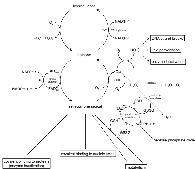
Figure 2. schematic overview of the redox cycle of quinones, the damage that can be induced by the radicals that are formed, and defense mechanisms of the host (reviewed in (19)).
