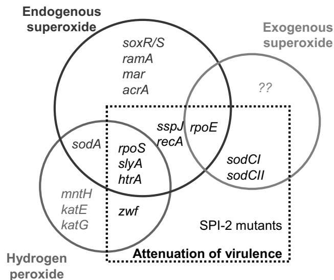
Figure 3. Classification of Salmonella mutants by in vitro and in vivo phenotype. Mutants that are sensitive to exogenous superoxide generated by the host NADPH-oxidase, endogenously produced superoxide and hydrogen peroxide are shown, and the consequences for virulence in mice are indicated. soxR/S , ramA , mar , acrA and oxyR encode transcriptional regulators; sodC/I and sodCII encode periplasmic copper-zinc superoxide dismutases; sodA encodes the cytoplasmic manganese superoxide dismutase; zwf encodes the glucose 6-phosphate dehydrogenase; htrA encodes a periplasmic protease; rpoE encodes an "extracytoplasmic function" sigma factor; rpoS and slyA encode transcriptional regulators; recA encode a recombinase important for DNA repair; sspJ encodes a periplasmic protein that interferes with superoxide levels; Spi2 is the pathogenicity island of Salmonella that contains genes encoding the second type-III secretion system.
