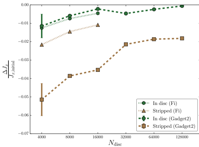
Fig. 6. Angular momentum lost from the disc during the final 1000 yr in terms of the initial angular momentum of the disc for both Fi (dotted) and Gadget2 (dashed). The angular momentum loss associated with processes in the disc, e.g. accretion of ISM, angular momentum exchange between accreted ISM and original disc material, is plotted in green and angular momentum loss associated with ablation is shown in brown. We have omitted the angular momentum loss due to accretion onto the star, because it is insignificant (as discussed in Sect. 4.2).
