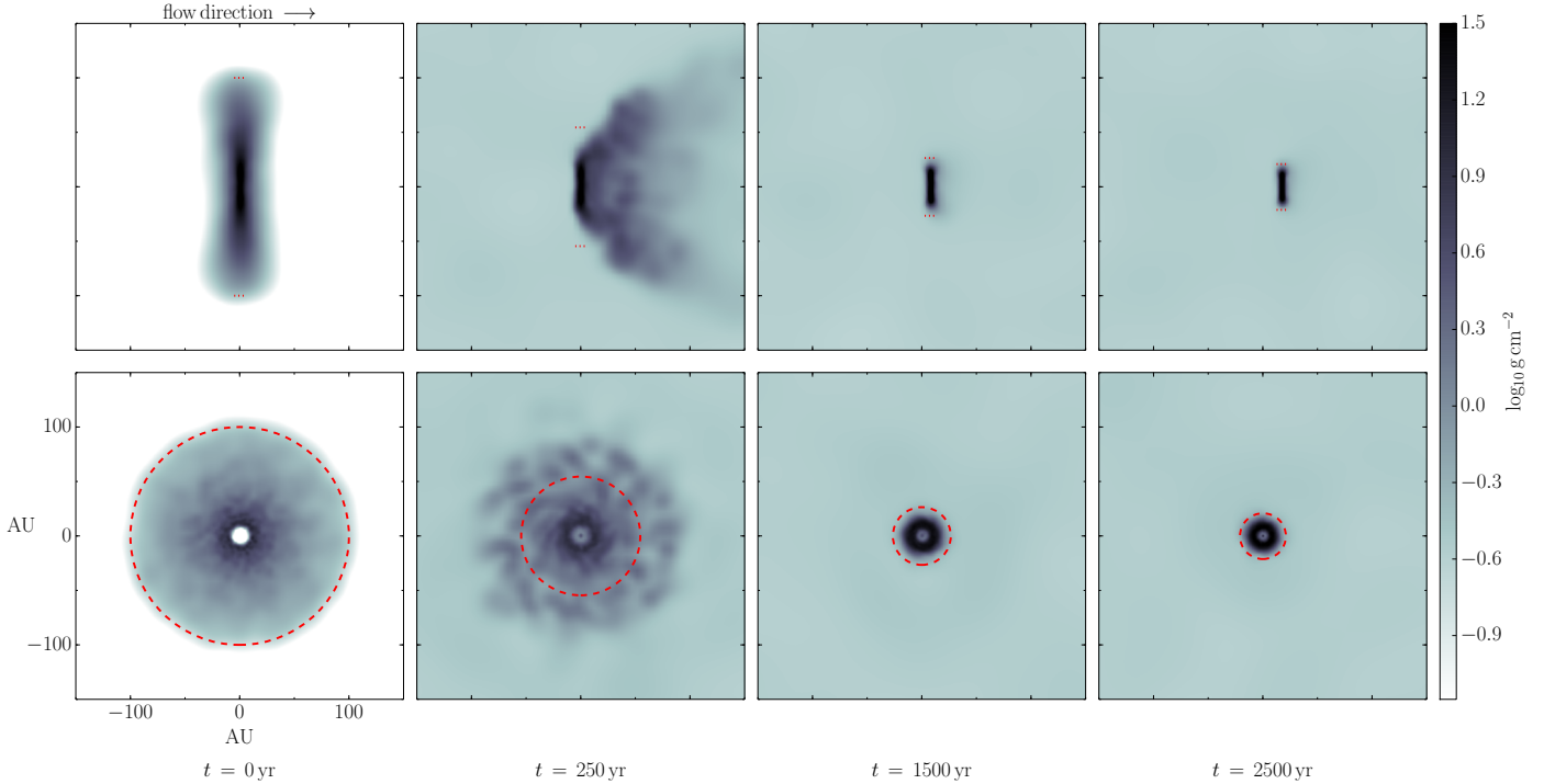
Fig. 3. Edge-on ( top row ) and face-on ( bottom row ) snapshots from the simulations with our reference model. The column density is shown in logarithmic scale and integrated along the full computational domain. The spatial scale is indicated in the bottom left and the flow direction on the top left . The red circle ( bottom row ) and dotted bars ( top row ) indicate the size of the disc as determined from its radius (see Sect. 3.3).
