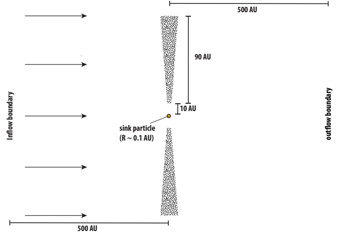
Fig. 1. Schematic overview of the numerical set-up.
