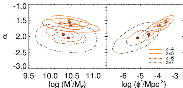
FIG. 11.— Confidence contours of the best-fit Schechter parameters for our fiducial (asymmetric-scatter) GSMFs at z = 4-7 at the 68% and 95% levels, showing that we can place reasonable constraints on \alpha . The best-fit Schechter parameters at z = 6-8 were derived with a log-normal prior on M^* , and their contours are denoted as dashed lines. z = 8 is omitted for clarity. The best-fit values are shown as filled circles.
