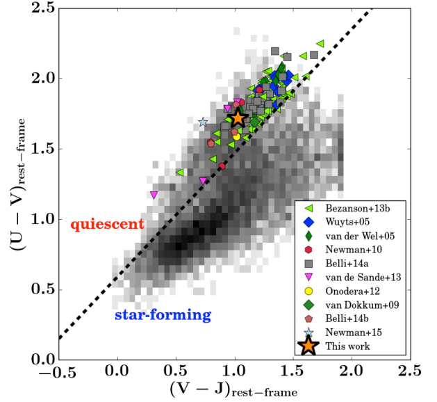
FIG. 2.— Rest-frame U - V color vs V - J color. Grey points are a redshift selected ( 1.5 < z < 2.5 ) comparison sample from the Ks-band selected UVISTA catalog (McCracken et al. 2012). The black dashed line is the colour selection implemented by van de Sande et al. (2015) to separate quiescent and star forming galaxies. Coloured points are a high redshift ( 0.6 < z < 2.3 ) sample compiled by van de Sande et al. (2015), with the literature sources indicated in the plot legend. Our object (orange star) sits on the UVISTA 1.5 < z < 2.5 red sequence, and within the locus of other high redshift, quiescent galaxies with measured stellar velocity dispersions.
