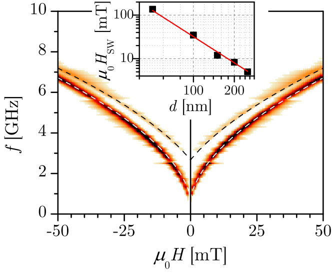
FIG. 4. Energy absorption in the broadband FMR experiments as a function of both magnetic field and frequency for the 200-nm-thick sample. Lines are fits to the theory for the main absorption line (lower curve) and for the first spin-wave mode (upper curve). The inset shows the dependence of the spin-wave field of the first mode H_{SW} , on the sample thickness d , (squares) together with the fit to the expected theoretical C/d^2 behavior (solid line).
