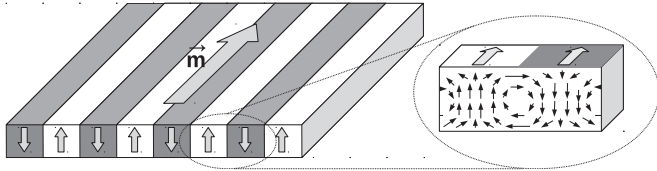
FIG. 1. Sketch of the magnetization directions in the weak stripe-domain phase of a film of permalloy. The main magnetization direction is given by \vec{m} . An alternating perpendicular is shown as gray and white areas. The zoom highlights the direction of the out-of-plane component and the variation of this component in a domain wall.
