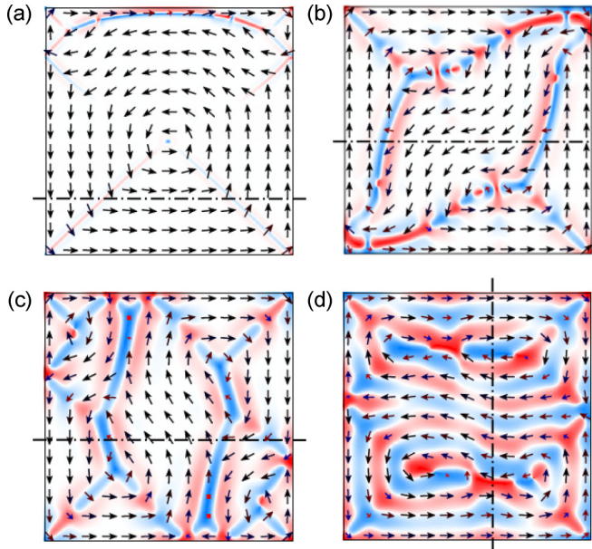
FIG. 8. Micromagnetic simulations (OOMMF software package) for square structures 4 \times 4 \mu\text{m}^2 with different thickness: 100 nm (a), 225 nm (b), 285 nm (c), and 345 nm (d). The images show the magnetization of the xy plane (film plane) at half of the thickness. The arrows represent the direction of the magnetization in the xy plane, while the color scale is for the magnetization component along z (red +z , blue -z ). In (a), out-of-plane components present along the diagonals of the square are barely visible. Dot-dash lines indicate the position of cross sections plotted in Fig. 9.
