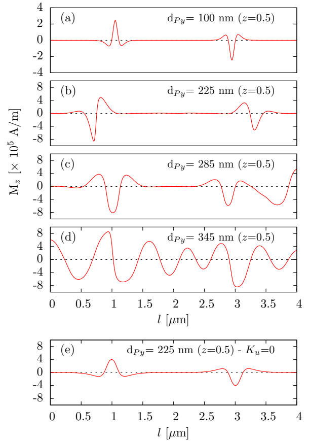
FIG. 9. (a)–(d) Cross sections of the images in Fig. 8 showing the perpendicular component of the magnetization, along the length of the section l . Position and direction of the cross section are shown in Fig. 8. The origin of the coordinates of the squares is the bottom-left corner. (e) Cross section for the same structure as in (b) but with no perpendicular anisotropy.
