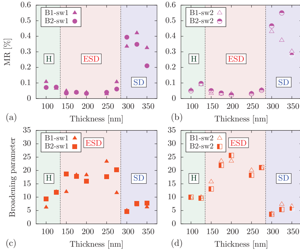
FIG. 7. Thickness dependence (a) and (b) of the magnetoresistance (MR) ratio and (c) and (d) of the broadening parameter for Py films patterned in 10- \mu\text{m} -wide bridges obtained from the R(H) curves given in Fig. 6. Two bridges (denoted B1 and B2) were patterned on each film. Panels (a) and (c) show the data obtained from the backward magnetic sweep (from positive to negative fields), for both structures; (b) and (d) are for the forward sweep (from negative to positive fields), for the same structures as in (a) and (c). The MR ratio is defined as 100 \times (R_{-20} - R_{\min})/R_{\min} (with R_{-20} = R(-20 \text{ mT}) and R_{\min} the minimum resistance value); the broadening parameter is the value of the area enclosed by the MR dip of the R(H) curves, after they are normalized by R(-20 \text{ mT}) and dip height. All the measurements are at 5 K. The dashed vertical lines divide the data in the three thickness regimes suggested by the measurements: homogeneous (H), emerging stripe domains (ESD), and stripe domains (SD).
