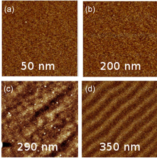
FIG. 2. Phase contrast images from magnetic force microscopy for full films in the three different thickness regimes: (a) 50 nm; (b) 200 nm; (c) 290 nm; and (d) 350 nm. (a), (b), and (d) are from the S1 series, (c) from S1b. Scan areas are 5 \times 5 \mu\text{m}^2 .
