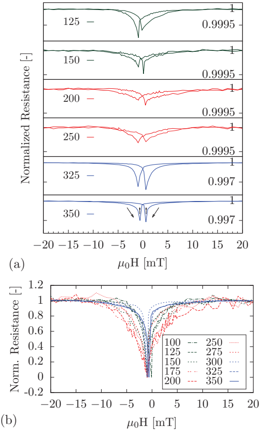
FIG. 6. (a) Magnetoresistance (MR) traces for patterned Py films (10- \mu\text{m} wide bridge), for different thicknesses denoted on the left (in nm). The curves are normalized by R(-20 \text{ mT}) . Note the change of scale when going from 250- to 325-nm thick structures. (b) All traces are shown together, normalized by R(-20 \text{ mT}) and the dip height. All measurements were taken at 5 K. In the bottom plot of (a) the arrows show the sweeping direction of the two curves; see details in the text.
