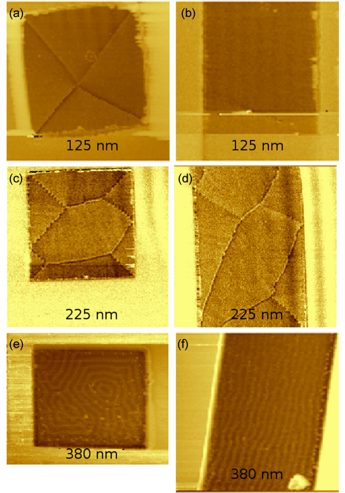
FIG. 3. Phase contrast images from magnetic force microscopy for patterned Py in the three different thickness regimes. (a) and (b) 125 nm; (c) and (d) 225 nm from the S3 series; and (e) and (f) 380 nm from the S3b series. Structures in (a) and (c) are squares 10 \times 10 \mu\text{m}^2 ; (e) is 10 \times 9 \mu\text{m}^2 . In (b), (d), and (f) a portion of a 10\text{-}\mu\text{m} wide bar is shown; scan ranges are 15 \times 15 \mu\text{m}^2 for (a), (c), (d), and (f), 14 \times 14 \mu\text{m}^2 for (b), and 15 \times 12 \mu\text{m}^2 for (e).
