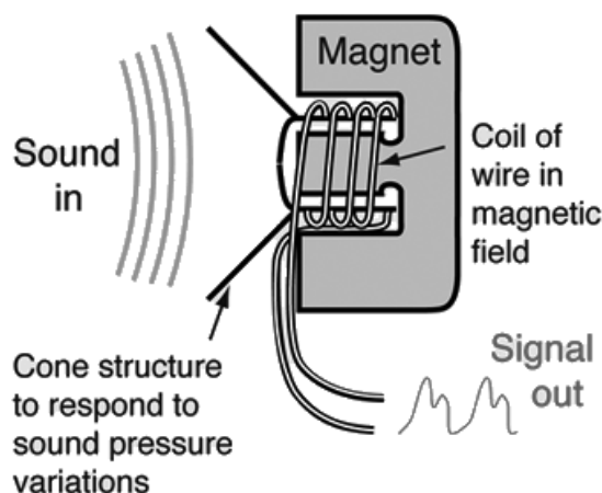
Dynamic microphone
