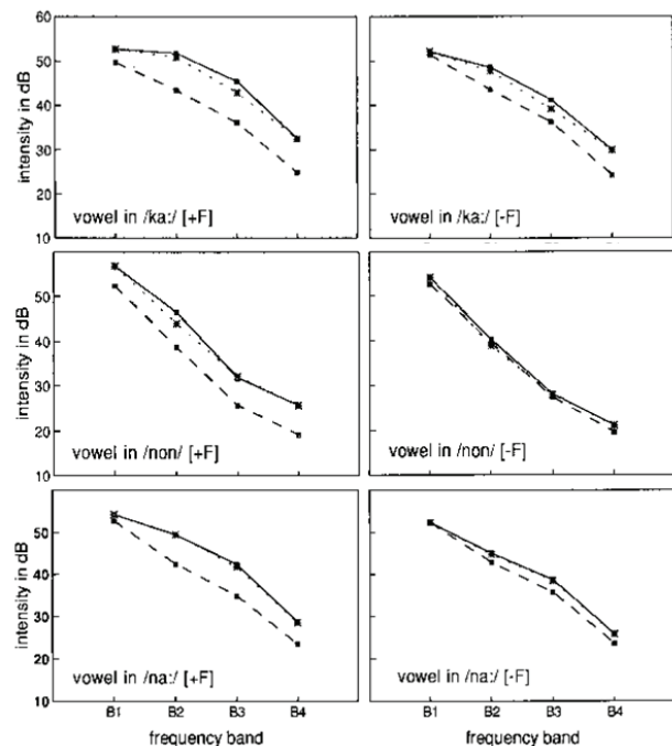
Figure 4. Effects of sentence (left column) and word (right column) stress on spectral tilt. Intensity (in dB) is plotted for four frequency bands (B1: < .5 KHz, B2: .5 - 1 KHz, B3: 1 - 2 KHz, B4: 2 - 4 KHz). Further see text.
