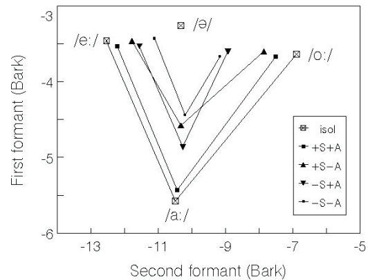
Figure 5. F_1 and F_2 (Bark) of three Dutch tense peripheral vowels produced by 15 male speakers in five stress conditions (see text, after [17]).
