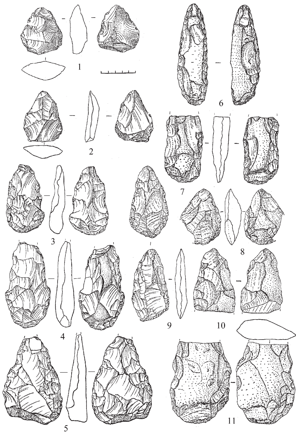
Figure 4.5 Bifaces from Upper Acheulian sites in the northwestern Caucasus: Sredniy Kbadjob (1, 2), Fortep'yanka (3), Abadzeb (4, 5), and Abin (6-11).
