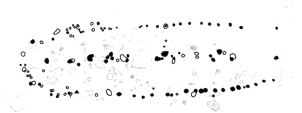
Fig. 7. The two-aisled house of Noordwijk dated to c. 1850 BC. Reconstruction of the author on the basis of the published plan (after Van Heeringen, Van De Velde & Van Amen, 1998: fig 11a). The closed postholes are deeper than 10 cm, the open postholes less than 10 cm deep.
