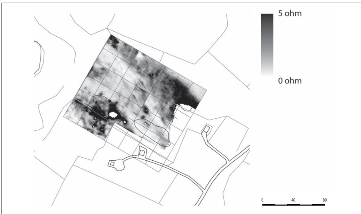
Fig. 5.14. Electric resistivity results at site G3 (village). The higher find densities recognised in the field survey are also indicated.
