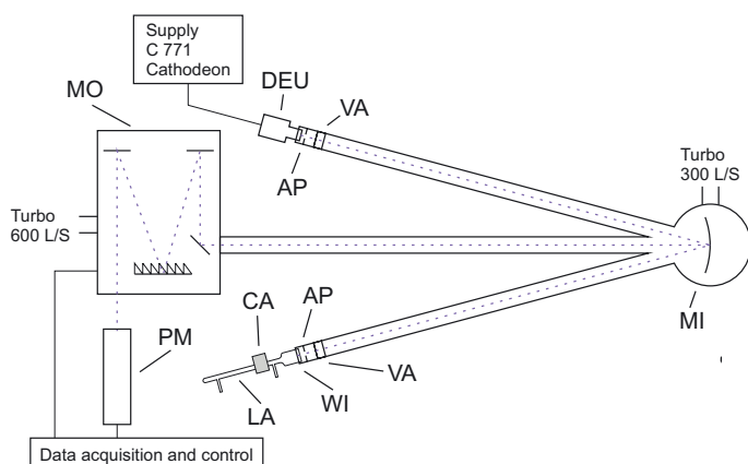
Fig. 2. Experimental set-up at the INP Greifswald for VUV measurements, (DEU): Physikalisch Technische Bundesanstalt (PTB) calibrated D 2 lamp, (AP): Aperture, 0.6 mm (diameter), (VA): Valve, (MI): Mirror, f = 1.5 m, (WI): MgF 2 window, (PM): Photomultiplier, (MO): VUV-Monochromator (VM-505 Acton Research); 0.5 m, 1200 g/mm, (LA): Microwave Discharge Hydrogen-flow Lamp, (CA): Microwave Evenson cavity.
