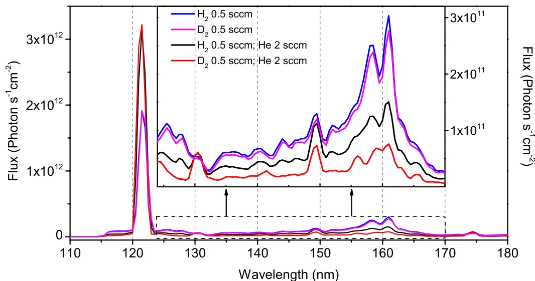
Fig. 3. VUV spectra in the 110–180 nm range of a T-type geometry MDHL, the H_2/D_2 partial pressure is kept at 0.41 mbar. The effect of adding helium with the H_2 or D_2 is clearly shown. Photon flux ( y -axis) estimations are based on NIST photodiode measurements. Emission at \sim 130 , \sim 149 , and \sim 175 nm indicate traces of oxygen and nitrogen.
