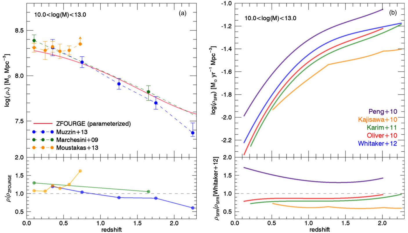
Figure 7. Panel (a) shows the buildup of stellar mass density in the range 10 < \log(M/M_\odot) < 13 as measured from multiple stellar mass functions. Below, the ratio of the measured stellar mass density relative to ZFOURGE is shown. The buildup of stellar mass varies between observations by a factor of about two, and ZFOURGE is comparable to other stellar mass functions in this respect, although it does measure a higher mass density in low-mass galaxies. In panel (b), we show the global star formation rate in galaxies with 10 < \log(M/M_\odot) < 13 as calculated from different observed star-forming sequences. Below, we show the ratio of the measured global star formation rate relative to that implied by the Whitaker et al. (2012) star-forming sequence. The global star formation rates also vary by a factor of \sim 2 , and the Whitaker et al. (2012) star-forming sequence is comparable to other observed star-forming sequences.
