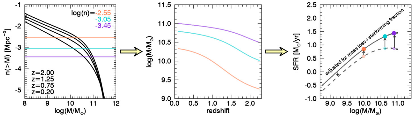
Figure 5. This figure describes the procedure to construct a star-forming sequence that is precisely consistent with the growth of the stellar mass function, under the assumptions that mergers are negligible and there is no scatter in star formation rates. In this case, galaxies evolve along lines of constant number density (Leja et al. 2013). For a given number density, this allows us to derive a relationship between redshift and stellar mass from \phi(M, z) . It is straightforward to convert this into \dot{M}(M) , as shown schematically above. We convert \dot{M}(M) into star formation rates by applying the inverse of the corrections for quiescent galaxies and passive stellar evolution shown in Figure 2.
