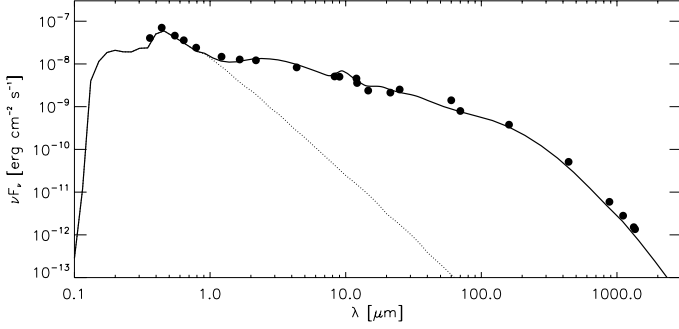
Fig. A.1. Spectral energy distribution (black line) of our best fit model, compared to dereddened photometry ( A_V = 0.3 , Q11) from the literature (Q11, Tilling et al. 2012; Cutri et al. 2011; Ishihara et al. 2010; Egan et al. 2003; Helou & Walker 1988). The stellar photosphere is shown as the thin dashed line.
