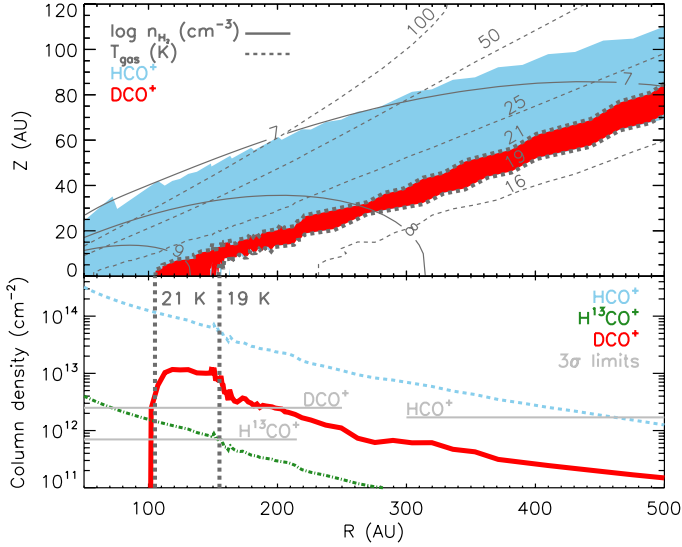
Fig. 3. Top: regions of non-zero HCO + (blue) and DCO + (red) abundance, overlaid with contours indicating the hydrogen density (solid gray lines) and temperature (dashed gray lines). The 19 and 21 K contours are shown with a thick dark gray line. The region containing HCO + is bounded on the upper and lower sides by CO photodissociation and by freezeout at 19 K, respectively. The DCO + region is bounded by the temperature range 19–21 K. Bottom: the column density of HCO + and its isotopologues (colored lines), with the 19 K CO snowline indicated by the thick dark gray dashed line. The broad plateau of the DCO + column density from ~110–150 AU explains the ring morphology seen in line emission. The 3 \sigma line sensitivities (from Sect. 3.2) are shown with the horizontal gray lines.
