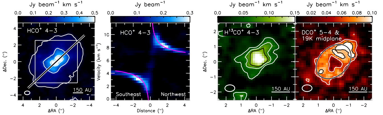
Fig. 1. Left: integrated emission map of HCO + (blue) from 0–12 km s -1 with contours showing 3, 10, and 17 \sigma emission ( \sigma = 25 mJy beam -1 km s -1 ). The white-bordered black line shows the positions from which we constructed the position–velocity diagram ( middle-left ), and the gray box shows the smaller region for which we show H 13 CO + and DCO + line emission ( middle-right and right ). Middle-left: the HCO + position–velocity diagram. The magenta curves show the Keplerian velocity profile for an assumed stellar mass of 2.3 M_{\odot} , disk inclination of 44°, and systemic velocity of 5.8 km s -1 . Middle-right: integrated emission map of H 13 CO + (green) from 0.8–10.4 km s -1 with contours showing 3, 5, and 7 \sigma emission ( \sigma = 14 mJy beam -1 km s -1 ). Right: integrated emission map of DCO + (red) from 0.8–10.4 km s -1 with contours showing 3 and 5 \sigma emission ( \sigma = 18 mJy beam -1 km s -1 ). The 19 K contour of the midplane temperature at a radius of 155 AU in the model disk is overlaid on the DCO + emission using a white-bordered black ellipse. In the maps of integrated emission, the \sim 0''.65 \times 0''.44 beam is shown in the lower left, while a scale is shown in the lower right.
