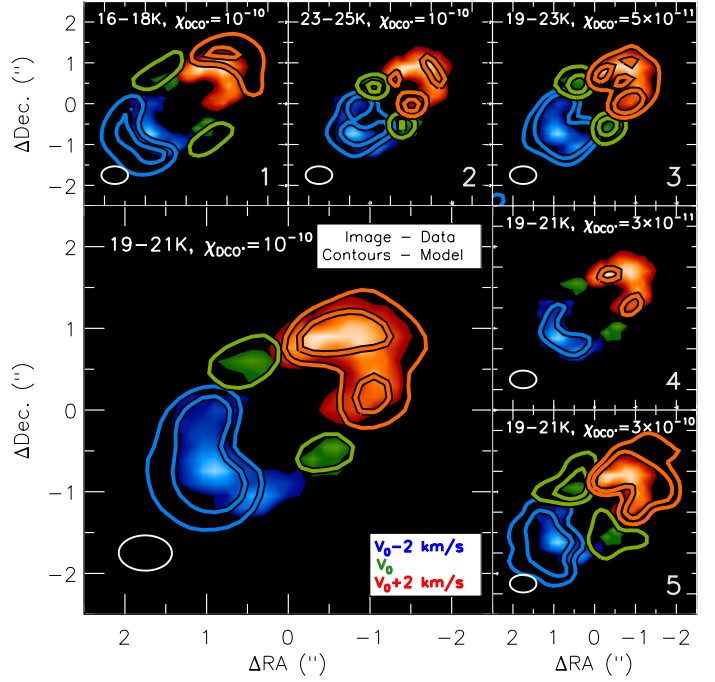
Fig. 2. Comparison of integrated intensities of our DCO + models (contours, 3 and 5 \sigma , \sigma = 15 mJy beam -1 km s -1 ) to the observations (image, colors show intensities from 3 \sigma ). Colors indicate the velocities the zeroth moment maps. Clockwise from the upper left, small figures show: 1) decreasing T_{low,DCO^+} and T_{high,DCO^+} by 3 K, 2) raising T_{low,DCO^+} and T_{high,DCO^+} by 4 K, 3) broadening the temperature range from 2 K to 4 K, with \chi_{DCO^+} halved to maintain the same total DCO + J = 5-4 line flux, 4) reduction of \chi_{DCO^+} by a factor of 3, and 5) raising \chi_{DCO^+} by a factor of 3.
