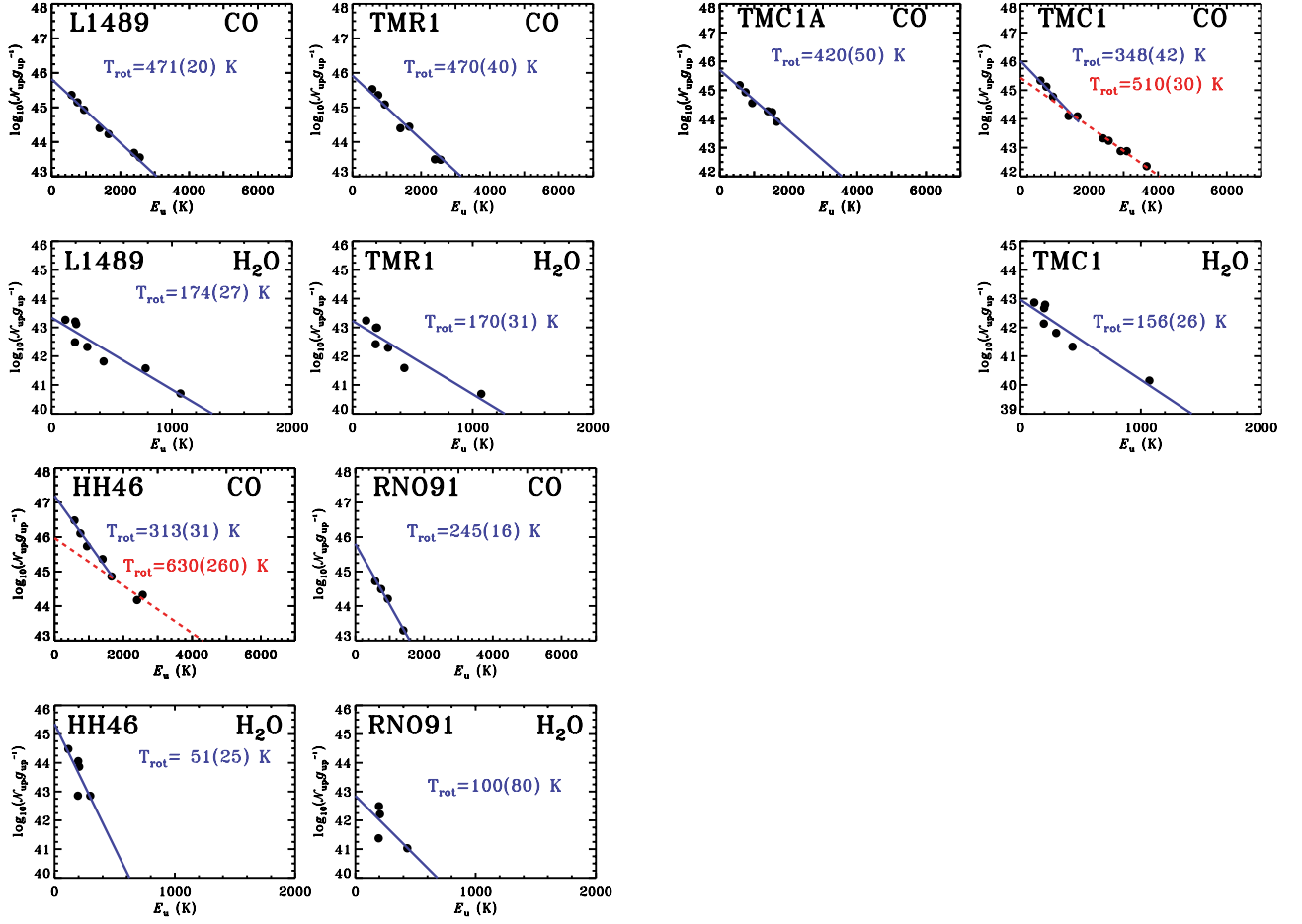
Fig. F.2. Rotational diagrams of CO H 2 O for Class I sources. Blue lines show linear fits to the data. The corresponding rotational temperatures are given. Errors associated with the fit are shown in the brackets. Warm components only are seen towards L1489, TMR1 and TMC1A in our diagrams.
