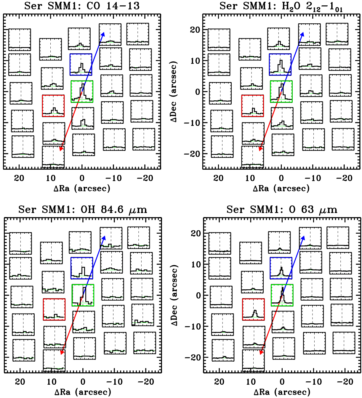
Fig. J.7. Ser SMM1 maps in the [OI] ^3\text{P}_1 - ^3\text{P}_2 line at 63.2 \mu\text{m} , the H 2 O 2 12 –1 01 line at 179.5 \mu\text{m} , the CO 14–13 at 186.0 \mu\text{m} , and the OH ^2\Pi_{3/2} J = 7/2 - 5/2 line at 84.6 \mu\text{m} .
