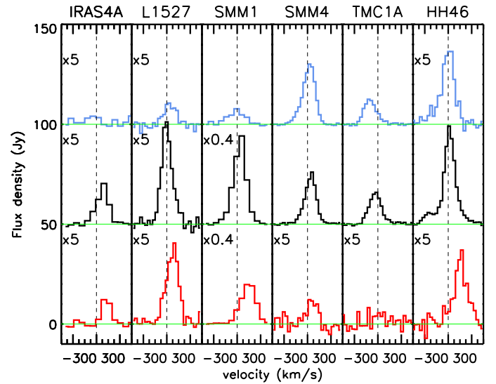
Fig. 6. Velocity shifts and high-velocity line wings in the [O I] line at 63.2 \mu\text{m} for NGC 1333-IRAS4A, L1527, Ser SMM1, SMM4, TMC1A, and HH46. Selected blue outflow, on-source and red outflow positions are shown for each object from top to bottom in velocity range from -300 to 300 \text{ km s}^{-1} . The black dashed line shows the laboratory wavelength of [O I].
