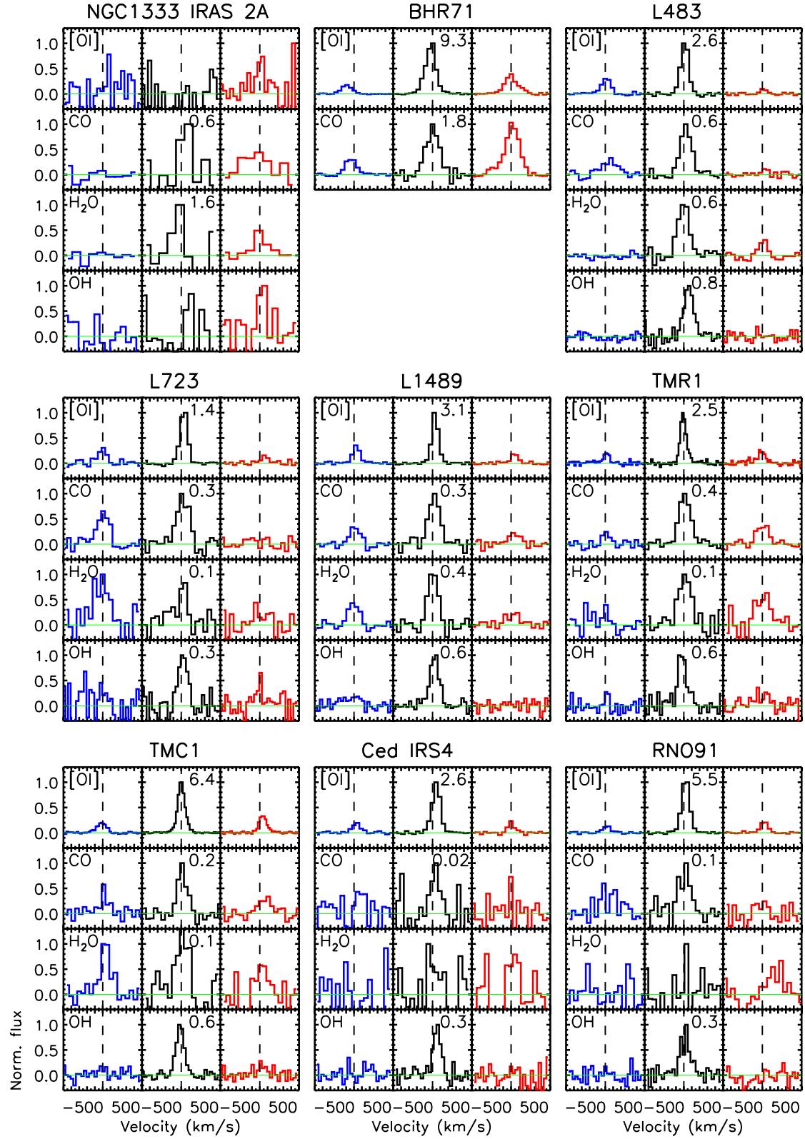
Fig. D.2. The same as Fig. D.1 but for the compact sources.
