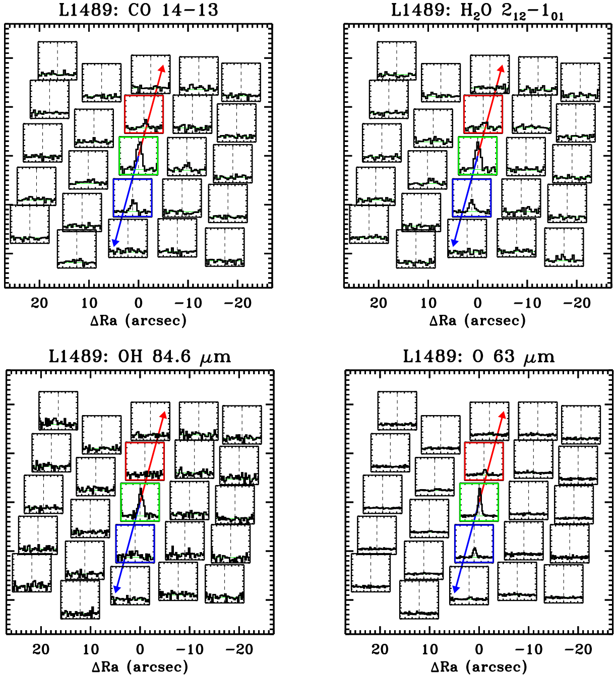
Fig. J.11. L1489 maps in the [O I] ^3\text{P}_1 – ^3\text{P}_2 line at 63.2 \mu\text{m} , the H 2 O 2 12 –1 01 line at 179.5 \mu\text{m} , the CO 14–13 at 186.0 \mu\text{m} , and the OH ^2\Pi_{3/2} J = 7/2 – 5/2 line at 84.6 \mu\text{m} .
