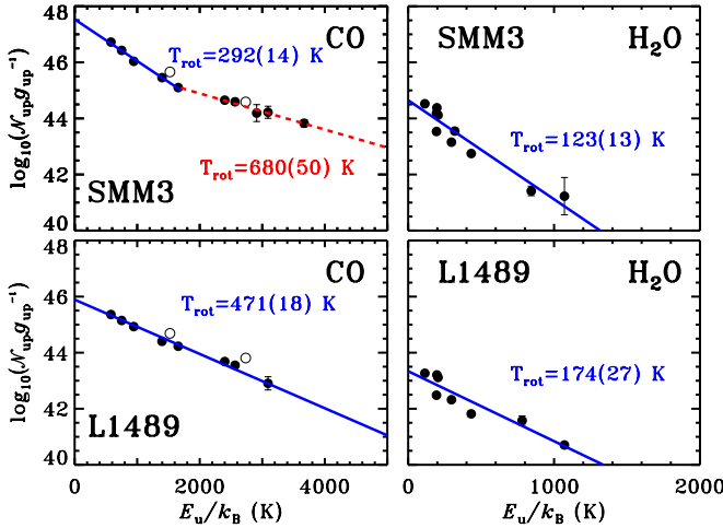
Fig. 7. CO (left panel) and H 2 O (right panel) rotational diagrams for Ser SMM3 (Class 0) and L1489 (Class I) calculated using the total flux in lines measured in the PACS field-of-view. The base 10 logarithm of the number of emitting molecules from a level u , N_u , divided by the degeneracy of the level, g_u , are written on the Y-axis. Two-component fits in the CO diagrams cover the transitions below and above E_u/k_B \sim 1700 K (CO 24–23) for the “warm” and “hot component” (see text). Each data point corresponds to one observed transition of a molecule. The limited number of lines observed in the line spectroscopy mode is responsible for the gaps in the otherwise linearly spaced CO diagrams. The error bars reflect the uncertainties in the fit.
