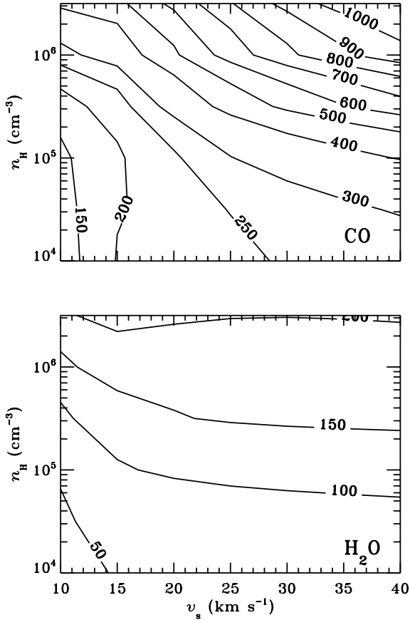
Fig. 13. Rotational temperature of CO ( top ) and H 2 O ( bottom ) as a function of different shock velocities and pre-shock densities from the shock model results of Kaufman & Neufeld (1996). The rotational temperature is calculated from J = 15-14 to 25-24 for CO and for the eight H 2 O lines commonly observed in this sample.
