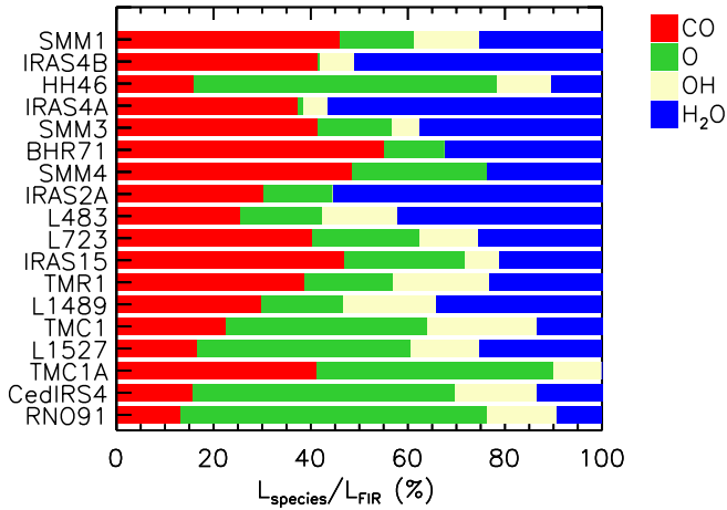
Fig. 8. Relative contributions of CO (red), [O I] (green), OH (yellow) and H 2 O (blue) to the total far-IR gas cooling integrated over the entire PACS array are shown from left to right horizontally for each source. The objects are in the sequence of decreasing total gas far-IR cooling, L_{\text{FIR}} . Note that OH cooling is not available for BHR71 and Ser SMM4 and not measured in NGC 1333-I2A. Water cooling is not calculated for TMC1A.
