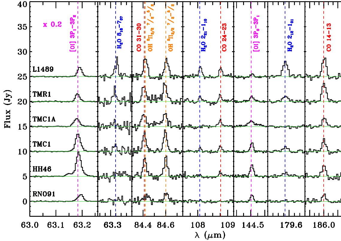
Fig. 2. Same as Fig. 1 but for Class I sources.
