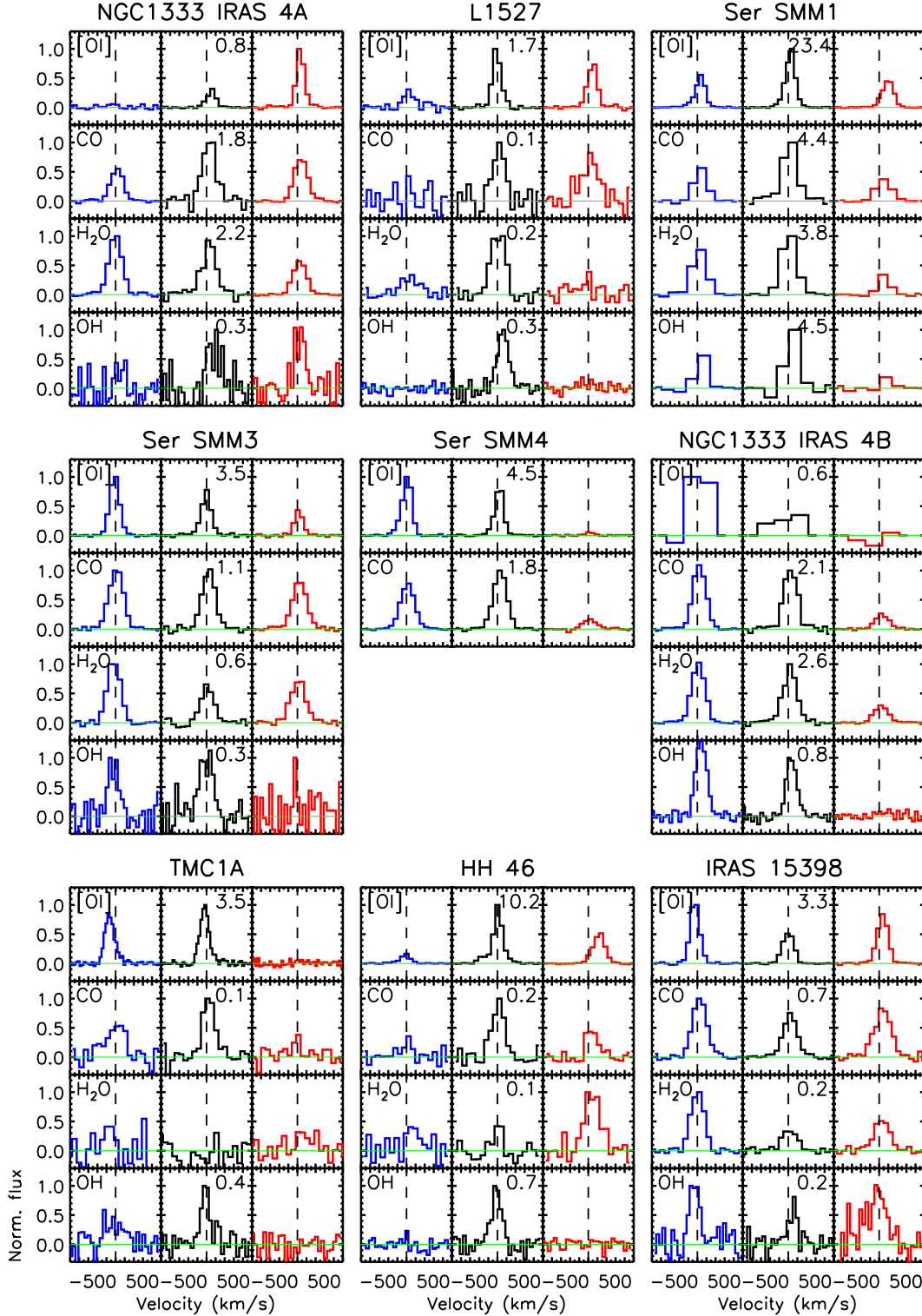
Fig. D.1. Spectra of the [O I] 63.2 \mu m, CO 14–13 186.0 \mu m, H 2 O 2 12 –1 01 179.5 \mu m, and OH 84.6 \mu m lines in the selected blue outflow, on-source and red outflow positions (marked with blue, green and red frames around the spaxels e.g. in Fig. 3) for the extended sources (see Sect. 3.2). The figure shows relative emission at different positions for each species separately. Measured line fluxes at central spaxel position in units of 10^{-20} W cm -2 are written next to the corresponding spectra.
