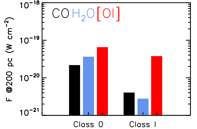
Fig. 14. Median line flux of the CO 14–13, H 2 O 2 12 –1 01 , and [OI] 3 P 1 – 3 P 2 lines for Class 0 and I objects from our sample are shown from left to right for each class in black, blue and red, respectively.
