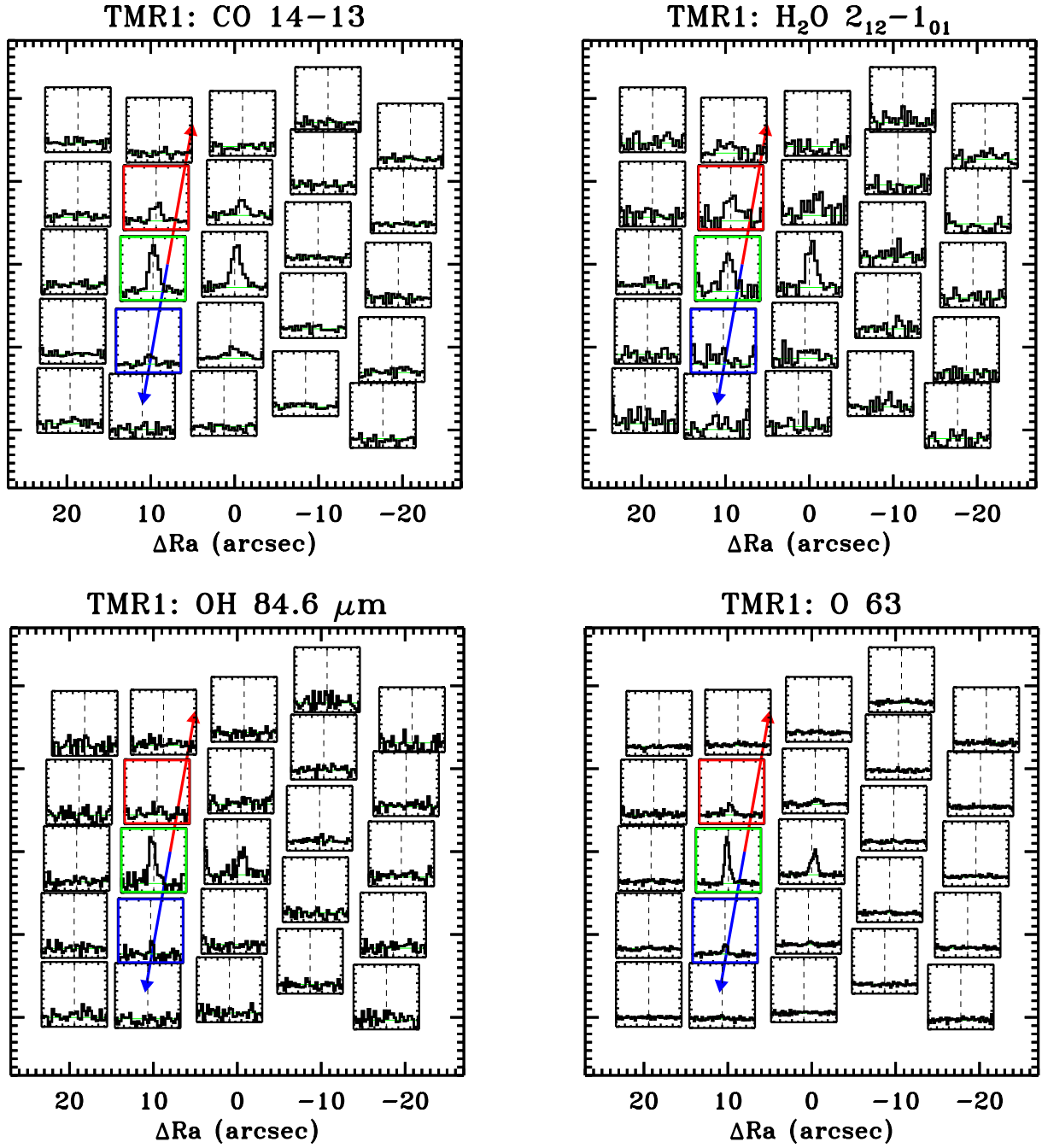
Fig. J.12. TMR1 maps in the [OI] ^3P_1 – ^3P_2 line at 63.2 \mu\text{m} , the H 2 O 2 12 –1 01 line at 179.5 \mu\text{m} , the CO 14–13 at 186.0 \mu\text{m} and the OH ^2\Pi_{3/2} J = 7/2 – 5/2 line at 84.6 \mu\text{m} .
