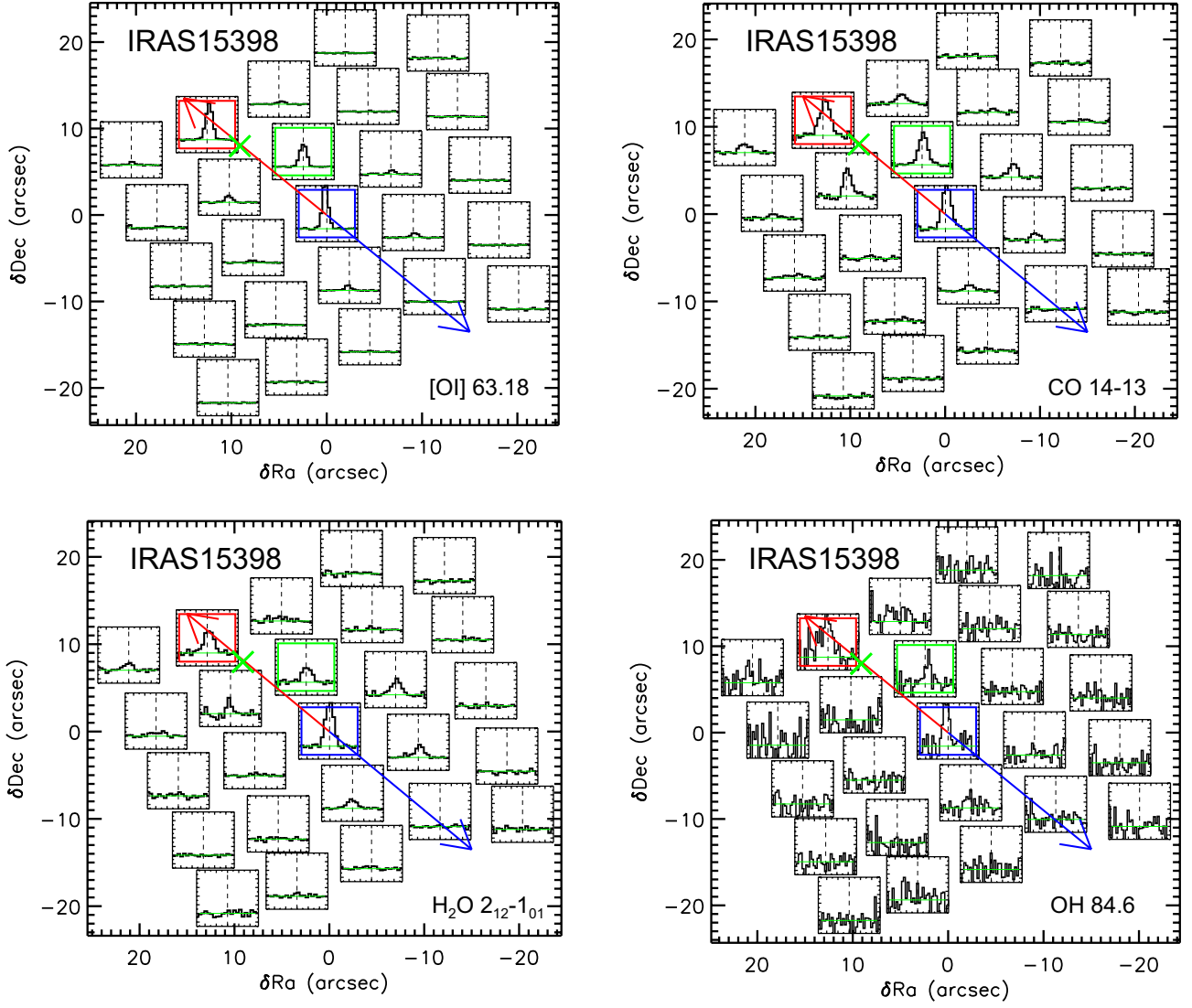
Fig. J.5. IRAS 15398 maps in the [OI] ^3P_1-^3P_2 line at 63.2\ \mu\text{m} , the H 2 O 2 12 -1 01 line at 179.5\ \mu\text{m} , the CO 14-13 at 186.0\ \mu\text{m} , and the OH ^2\Pi_{3/2}\ J = 7/2-5/2 line at 84.6\ \mu\text{m} . Green cross shows the on-source position.
