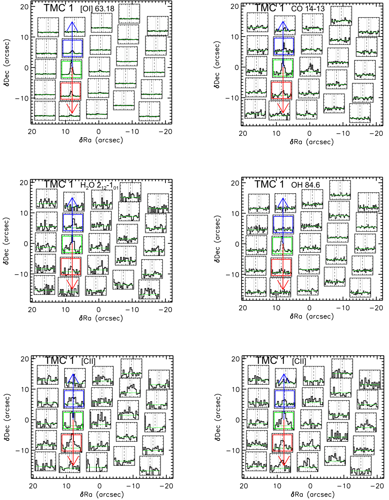
Fig. J.14. TMC1 maps in the [OI] ^3P_1-^3P_2 line at 63.2\ \mu\text{m} , the \text{H}_2\text{O}\ 2_{12}-1_{01} line at 179.5\ \mu\text{m} , the CO 14–13 at 186.0\ \mu\text{m} , and the OH ^2\Pi_{3/2}\ J = 7/2-5/2 line at 84.6\ \mu\text{m} . At the bottom, two nodes of [C II] observations are shown.
