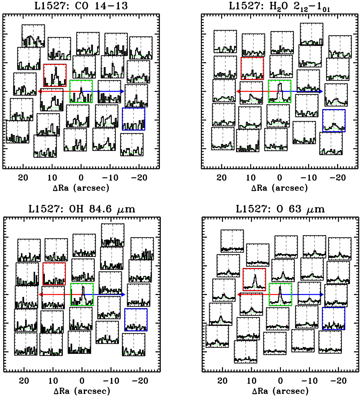
Fig. J.2. L1527 maps in the [O I] ^3\text{P}_1 – ^3\text{P}_2 line at 63.2 \mu\text{m} , the H 2 O 2 12 –1 01 line at 179.5 \mu\text{m} , the CO 14–13 at 186.0 \mu\text{m} , and the OH ^2\Pi_{3/2} J = 7/2 – 5/2 line at 84.6 \mu\text{m} .
