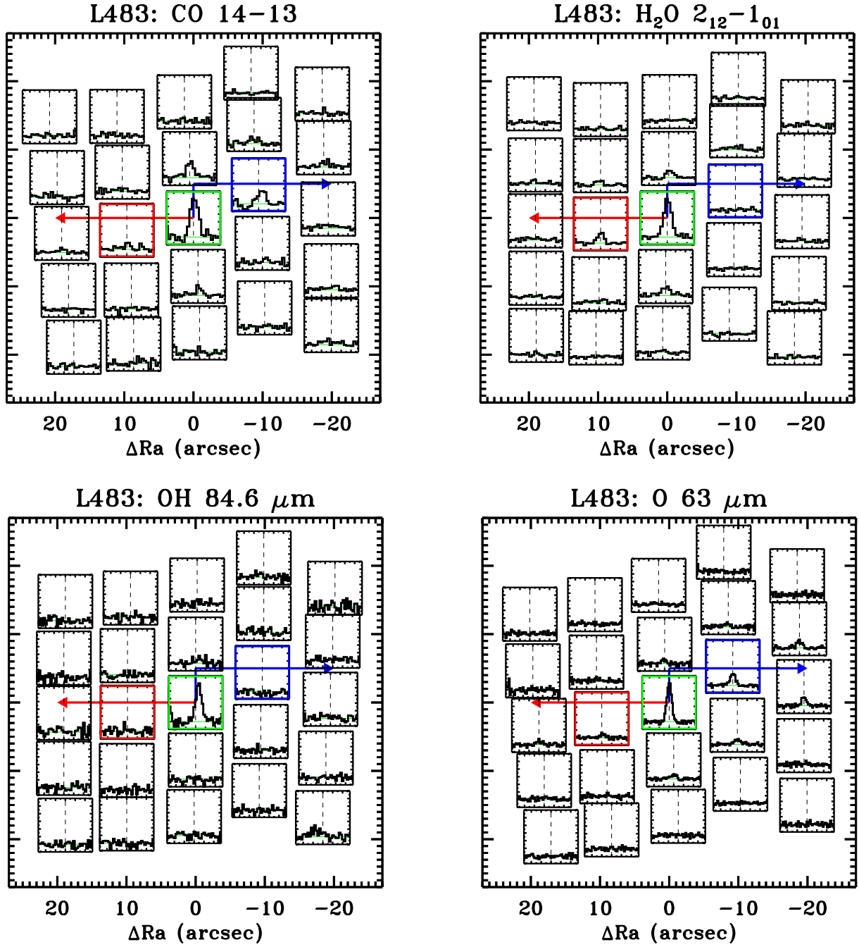
Fig. J.6. L483 maps in the [O I] ^3P_1-^3P_2 line at 63.2 \mu\text{m} , the H 2 O 2 12 -1 01 line at 179.5 \mu\text{m} , the CO 14-13 at 186.0 \mu\text{m} , and the OH ^2\Pi_{3/2} J = 7/2-5/2 line at 84.6 \mu\text{m} .
