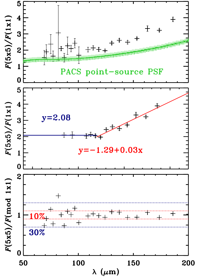
Fig. B.1. Illustration of the correction curve method. Top: CO fluxes of Serpens SMM1 measured over 5 \times 5 array divided by the central spaxel fluxes are plotted versus wavelengths. PACS PSF for a point source is shown in green. CO emission is clearly extended for this sources. Middle: best signal-to-noise measurements are used to make a fit to the data and derive the wavelength-dependent correction factors. Bottom: CO fluxes measured over 5 \times 5 array are divided by central spaxel measurements corrected for the extended emission using calculated correction factors are plotted versus wavelength. Accuracy longward \sim 100 \mu\text{m} is better than 10%, whereas the accuracy is \sim 30\% for short-wavelength lines ( \leq 100 \mu\text{m} ).
