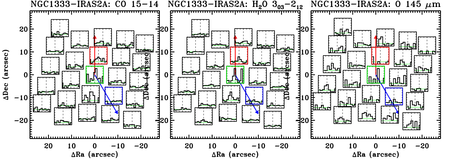
Fig. J.1. NGC 1333-IRAS2A maps in the CO 15–14 line at 173.6 \mu\text{m} , the H 2 O 3_{03} – 2_{12} line at 174.6 \mu\text{m} , and the [OI] ^3P_0 – ^3P_1 line at 145.5 \mu\text{m} .
