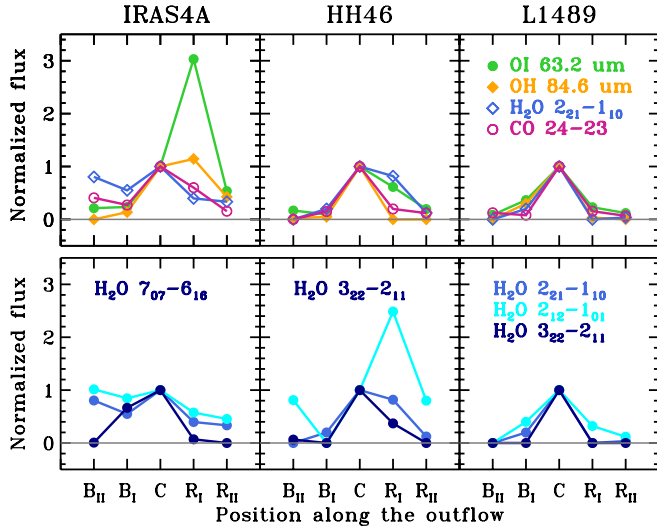
Fig. 5. Extent of line emission along the outflow direction for the selected molecular and atomic lines. Top panel: the [O I] 63.2 \mu\text{m} line (green filled circles), the OH 84.6 \mu\text{m} line (orange filled diamonds), the H 2 O 2 21 –1 10 line at 108 \mu\text{m} (blue empty diamonds), and the CO 24–23 line (violet empty circles) are shown for each object. Bottom panel: the H 2 O 2 21 –1 10 line at 108 \mu\text{m} (blue), the H 2 O 2 12 –1 01 line at 179 \mu\text{m} (light blue) are shown for all objects. Additionally, the H 2 O 7 16 –6 07 line at 71.9 \mu\text{m} is shown for IRAS4A and the H 2 O 3 22 –2 11 at 89.9 \mu\text{m} line is shown for HH46 and L1489 (all in navy blue). The X-axis shows the selected spaxel names along the outflow direction (see Fig. 3), whereas the Y-axis shows the flux normalized to the central spaxel (C) value.
