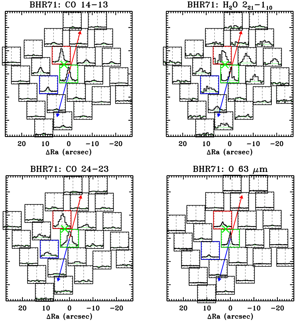
Fig. J.4. BHR71 maps in the [O I] ^3P_1-^3P_2 line at 63.2 \mu m , the H 2 O 2_{21}-1_{10} at 108.1 \mu m , the CO 14-13 at 186.0 \mu m , and the CO 24-23 at 108.7 \mu m .
