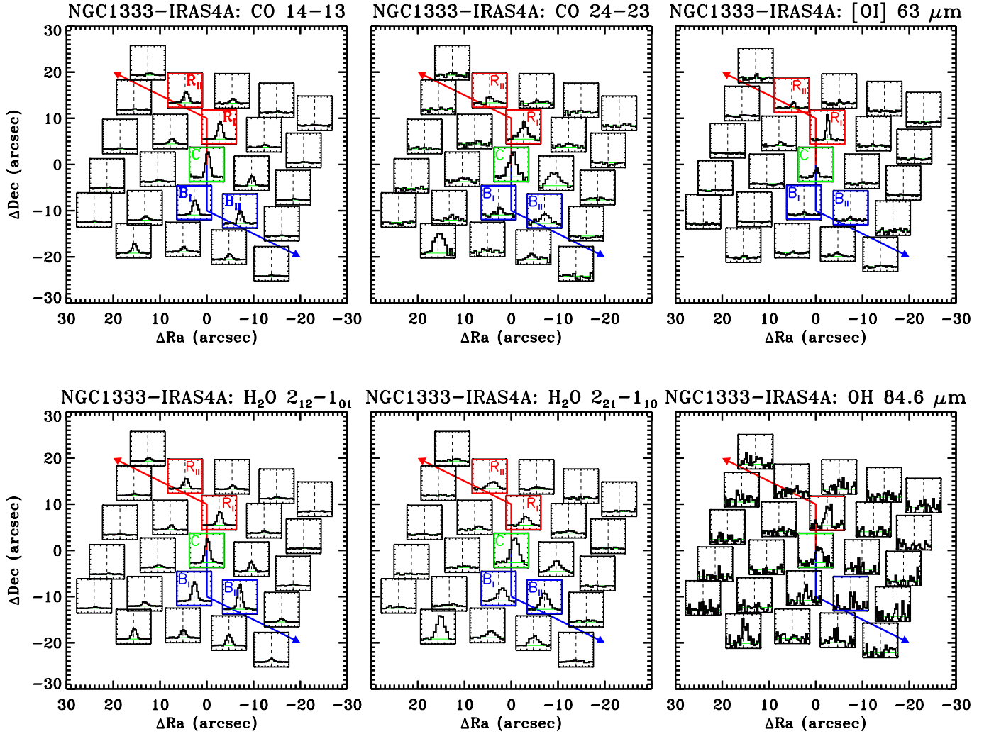
Fig. 3. PACS spectral maps of the Class 0 source NGC 1333-IRAS4A in the CO 14–13, CO 24–23, [OI] 63.2 \mu\text{m} , \text{H}_2\text{O} 2 12 –1 01 , \text{H}_2\text{O} 2 21 –1 10 and OH 84.6 \mu\text{m} lines. The center of each spaxel box corresponds to its position on the sky with respect to the pointed source coordinates from van Dishoeck et al. (2011) ; shown boxes are smaller than the actual spaxel sizes. Wavelengths in microns are translated to the velocity scale on the X-axis using laboratory wavelengths of the species and cover the range from -550 to 550 \text{ km s}^{-1} , except for the OH 84.6 \mu\text{m} lines where -400 to 400 \text{ km s}^{-1} is shown. The Y-axis shows fluxes normalized to the brightest spaxel on the map separately for each species in a range -0.2 to 1.2 . Outflow directions are drawn in blue and red lines based on CO 6–5 APEX CHAMP + sub-mm maps ( Yıldız et al. 2012 , and in prep.) that traces the warm entrained gas ( T \sim 100 \text{ K} ). Two red outflow ( R_I , R_{II} ), on-source (C) and blue outflow ( B_I , B_{II} ) spaxels are marked with letters. IRAS4A spectra at those positions in different species are shown in Appendix D. The contribution from NGC 1333-IRAS4B, located at (22.5'', -22.8'') with respect to IRAS4A, is seen in the S-E part of the map.
