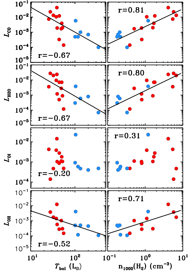
Fig. G.1. Correlations between bolometric temperature ( left column ) and envelope density at 1000 AU ( right column ) and (from top to bottom ): CO 14–13, H 2 O 2 12 –1 01 , [O I] at 63.18 \mu\text{m} , and OH 84.6 \mu\text{m} line luminosities.
