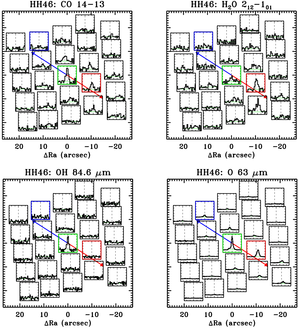
Fig. J.15. HH46 maps in the [O I] ^3P_1 – ^3P_2 line at 63.2 μm, the H 2 O 2 12 –1 01 line at 179.5 μm, the CO 14–13 at 186.0 μm and the OH ^2\Pi_{3/2} J = 7/2 – 5/2 line at 84.6 μm.
