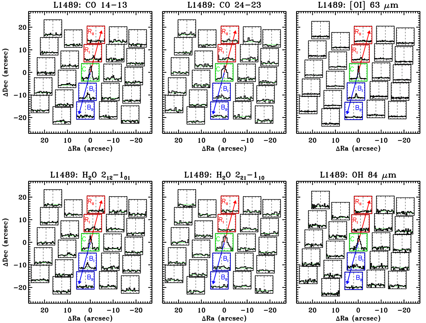
Fig. 4. The same as Fig. 3 but for the Class I source L1489.
