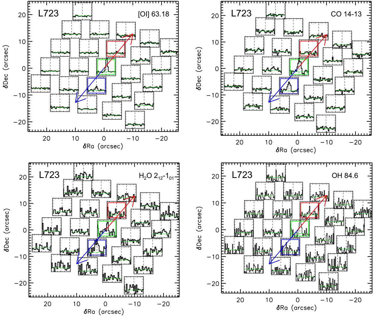
Fig. J.10. L723 maps in the [OI] ^3P_1-^3P_2 line at 63.2 \mu\text{m} , the H 2 O 2 12 -1 01 line at 179.5 \mu\text{m} , the CO 14-13 at 186.0 \mu\text{m} , and the OH ^2\Pi_{3/2} J = 7/2-5/2 line at 84.6 \mu\text{m} .
