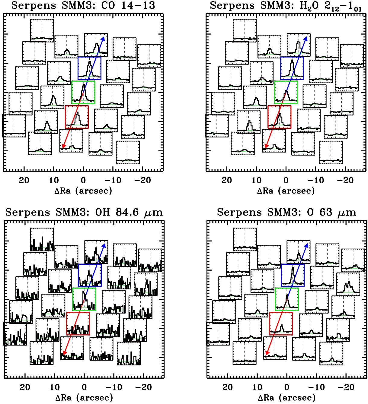
Fig. J.9. Ser SMM3 maps in the [O I] ^3\text{P}_1 – ^3\text{P}_2 line at 63.2 \mu\text{m} , the H 2 O 2 12 –1 01 line at 179.5 \mu\text{m} , the CO 14–13 at 186.0 \mu\text{m} , and the OH ^2\Pi_{3/2} J = 7/2 – 5/2 line at 84.6 \mu\text{m} .
