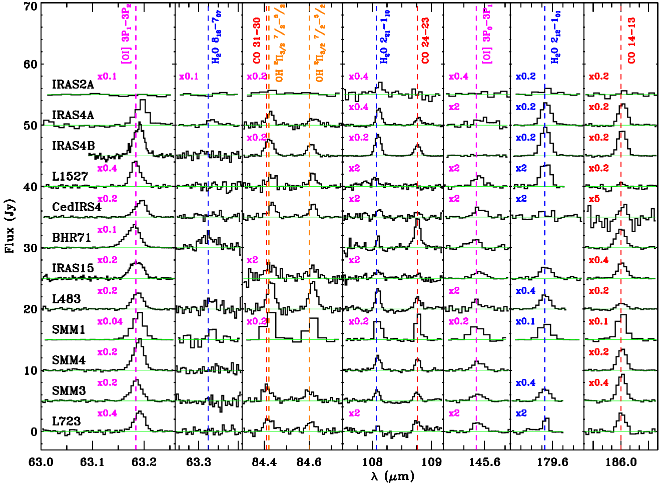
Fig. 1. Line survey of Class 0 sources at the on-source position. Spectra are extracted from the central spaxel only for the well-pointed sources (for mispointed sources see text) and continuum subtracted. No correction for point spread function is made. Dashed lines show laboratory wavelengths of [O I] (pink), OH (orange), CO (red), and H 2 O (blue). BHR71 and Ser SMM4 were not observed in all the lines within our program (see text).
