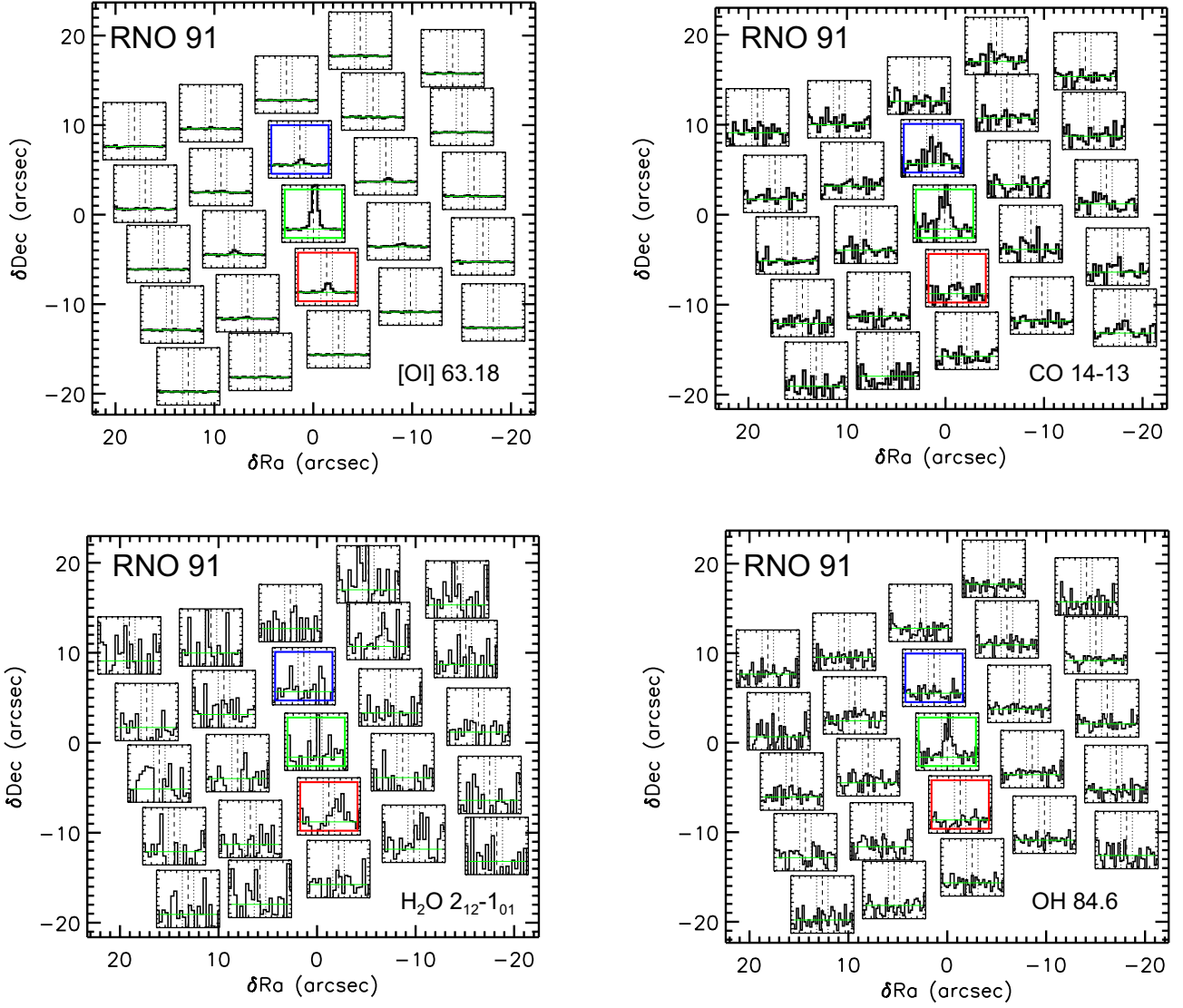
Fig. J.16. RNO91 maps in the [O I] ^3\text{P}_1 - ^3\text{P}_2 line at 63.2 \mu\text{m} , the \text{H}_2\text{O } 2_{12}-1_{01} line at 179.5 \mu\text{m} , the CO 14–13 at 186.0 \mu\text{m} , and the OH ^2\Pi_{3/2} J = 7/2 - 5/2 line at 84.6 \mu\text{m} .
