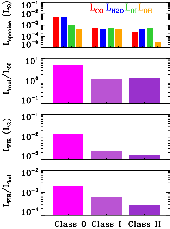
Fig. 15. Panel 1: median cooling in CO, H 2 O, OH, and [OI] lines for Class 0, I, and II objects are shown from left to right for each class in red, blue, orange and green colors, respectively. (Class II data from Podio et al. 2012.). Panel 2: evolution of the ratio of molecular and atomic cooling. Panel 3: evolution of the median total far-IR gas cooling. Panel 4: evolution of the median total far-IR gas cooling over bolometric luminosity.
