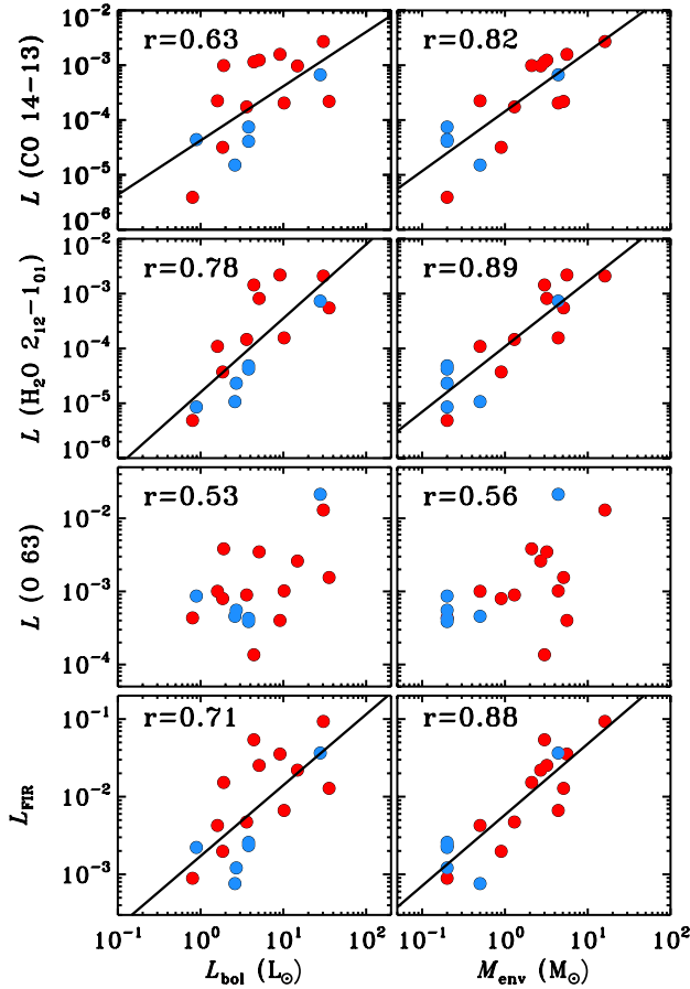
Fig. 10. Correlations of full array line emission with bolometric luminosity (left column) and envelope mass (right column) from top to bottom: CO 14–13, H 2 O 2 12 –1 01 , [O I] at 63.2 μm line luminosities, and total far-IR gas cooling L_{\text{FIR}} .
