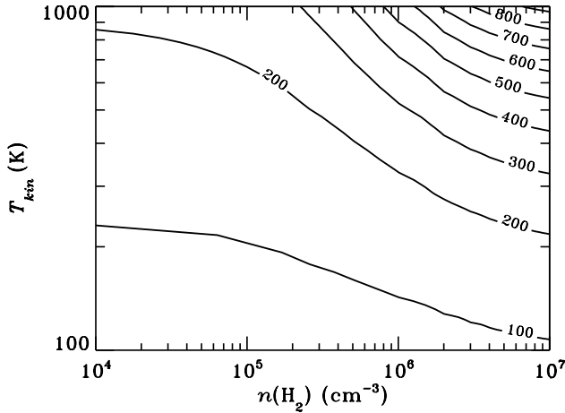
Fig. 12. CO rotational temperature T_{\text{rot}} from J = 15\text{--}14 to 25\text{--}24 as a function of density n_{\text{H}} and temperature of the emitting gas derived from non-LTE excitation calculations.
