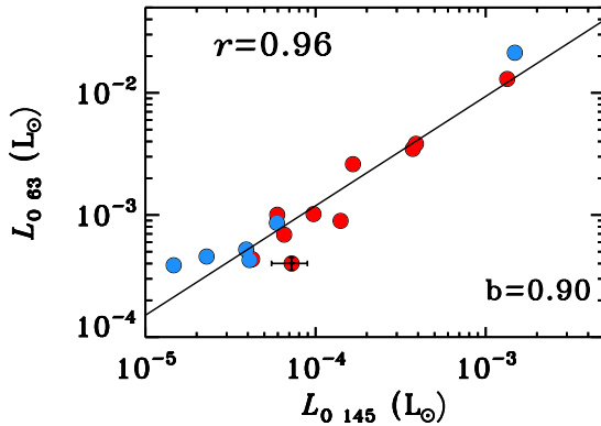
Fig. 11. Full array correlation between the [O I] line luminosities at 145 and 63 μm for 16 out of 18 objects (the [O I] 145 line is not detected in NGC 1333-IRAS2A and 4B). Class 0 sources are shown in red and Class I sources in blue. A typical error is shown on the NGC 1333-IRAS4A observation.
