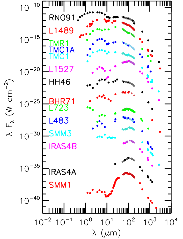
Fig. C.1. Spectral energy distribution shapes for most of our sources. Literature observations are shown as filled circles, whereas our PACS observations are marked with crosses and drawn in a different hue (see Table C.1). The maxima of the SEDs lie between 10^{-16} and 10^{-19} \text{W cm}^{-2} for all objects and thus, for better shape visualization, the SEDs are offset by several orders of magnitude. Objects are shown in the sequence of decreasing evolutionary parameter L_{\text{bol}}^{0.6}/M_{\text{env}} .
