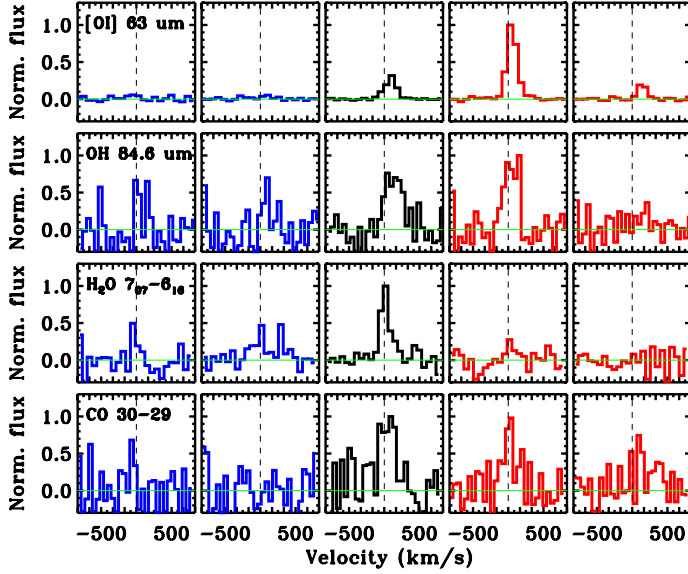
Fig. D.3. NGC 1333-IRAS4A spectra in the [OI] 63.2 \mu\text{m} line, the OH 84.6 \mu\text{m} line, the H 2 O 7 07 –6 16 line, and the CO 30–29 line. Two blue outflow, on-source and two red outflow positions are shown, corresponding to the colored spaxels in Fig. 3.
