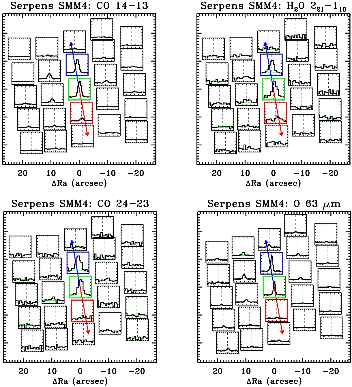
Fig. J.8. Ser SMM4 maps in the [OI] ^3P_1-^3P_2 line at 63.2 \mu m, the H 2 O 2_{21}-1_{10} at 108.1 \mu m, the CO 14–13 at 186.0 \mu m, and the CO 24–23 at 108.7 \mu m.
