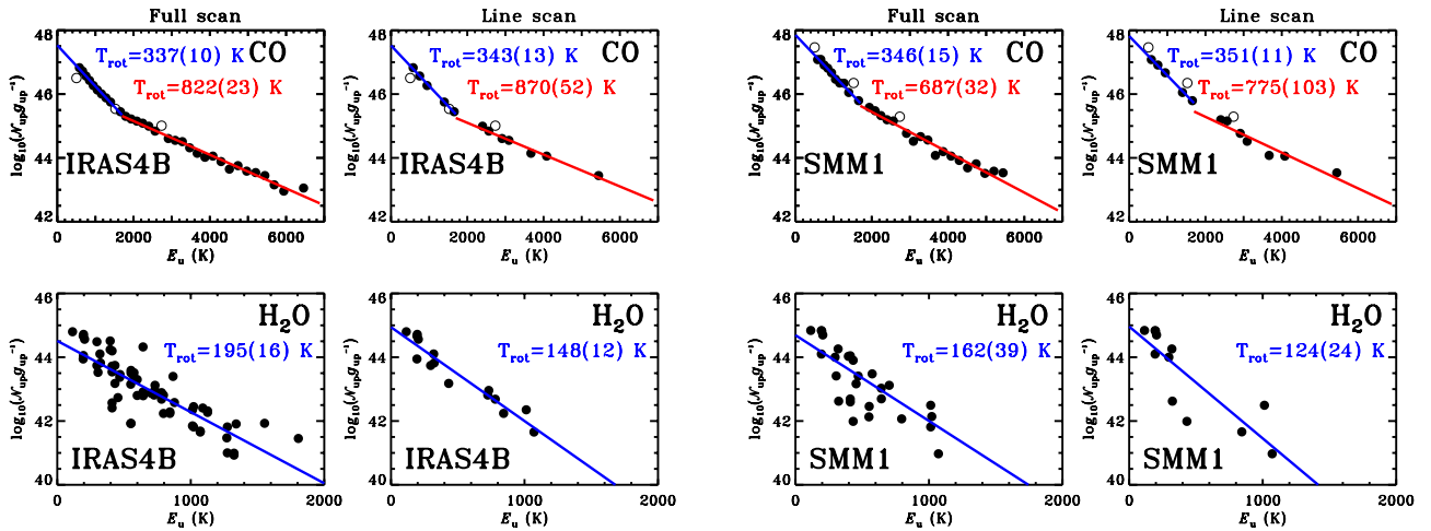
Fig. H.1. The CO and H 2 O rotational diagrams for NGC 1333-IRAS4B and Serpens SMM1. Both the full spectroscopy line and the selected lines observed in the line scan mode are shown. Two component fit is done to the CO diagram with the break at 1700 K (i.e. transitions J \geq 24 correspond to the warm component) and a single component fit to the H 2 O diagram. Errors associated with the fit are shown in the brackets.
