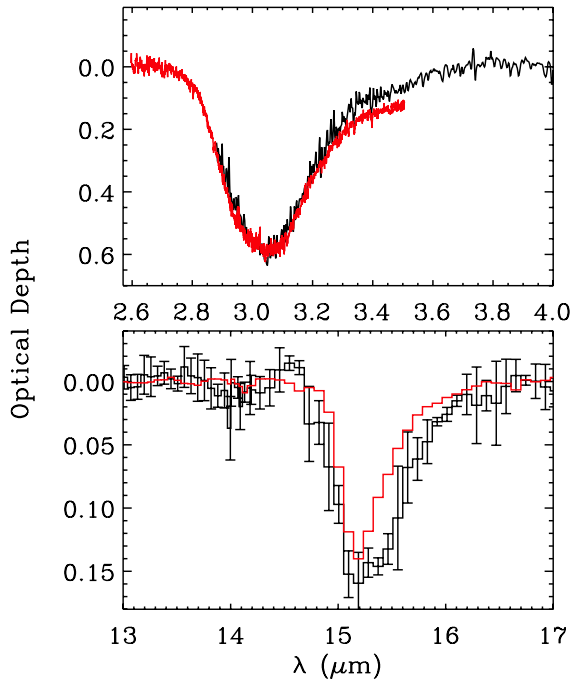
Figure 6. 3.0 \mu\text{m} \text{H}_2\text{O} (top panel) and 15 \mu\text{m} \text{CO}_2 (bottom) bands for the background stars 2MASS J15452747–3425184 (Lupus I; in black) and Elias 16 (TMC; in red). The spectra are scaled to the solid \text{H}_2\text{O} column density. The pronounced wing in the \text{CO}_2 bending mode toward 2MASS J15452747–3425184 may indicate a larger fraction of \text{H}_2\text{O} -rich ices (not further analyzed in this work).
