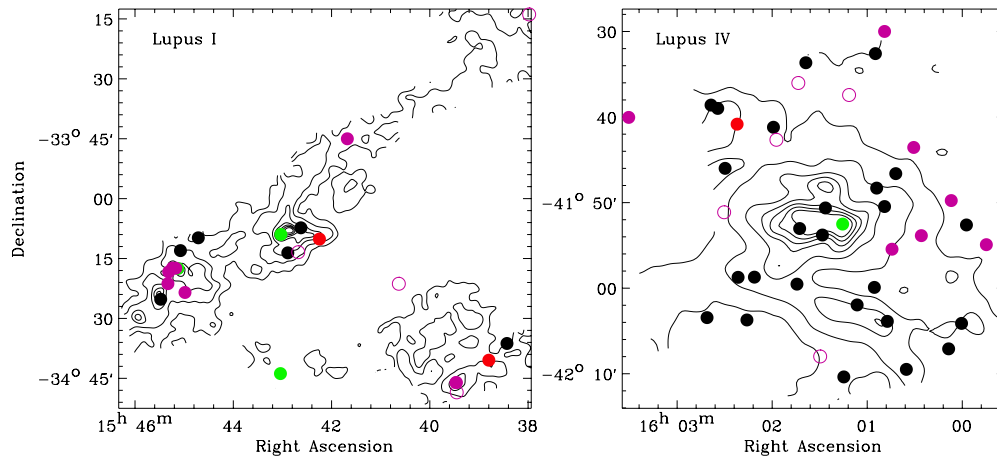
Figure 1. Background stars (black filled circles) observed toward the Lupus I (left panel) and Lupus IV (right) clouds, overplotted on extinction maps (Evans et al. 2007) with contours A_K = 0.25, 0.5, 1.0, 1.5, 2.0, 2.5, 3.0 mag (assuming A_V/A_K = 7.6 for R_V = 5.0 ; Cardelli et al. 1989). The red filled circles indicate Class I YSOs, green filled circles Flat spectrum YSOs, purple filled circles Class II YSOs, and purple open circles Class III YSOs (all from Merín et al. 2008). (A color version of this figure is available in the online journal.)
