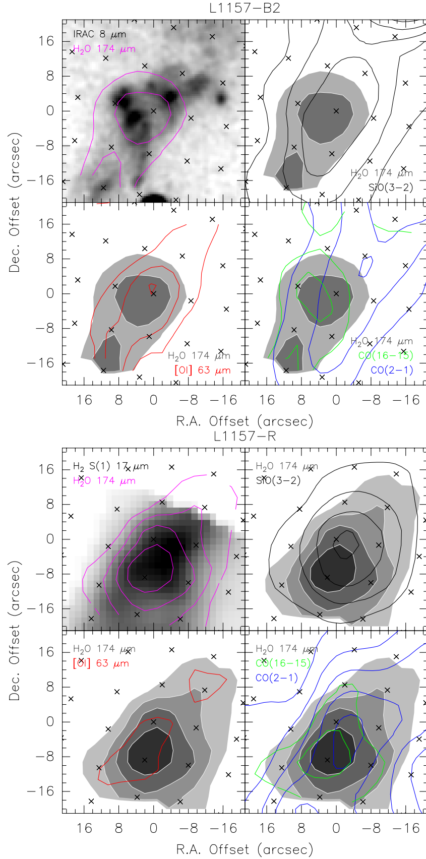
Fig. 3. Same as in Fig. 2, but for the L1157 outflow. Contours are displayed for IRAM-30 m CO(2–1) and SiO(3–2) emission (HPBW equal to 11'' and 18'', respectively) from Bachiller et al. (2001) and are traced in steps of 5\sigma , starting from 5\sigma . Spitzer -IRAC 8 \mu\text{m} emission and Spitzer -IRS H 2 S(1) emission at 17 \mu\text{m} from Neufeld et al. (2009) are shown.
