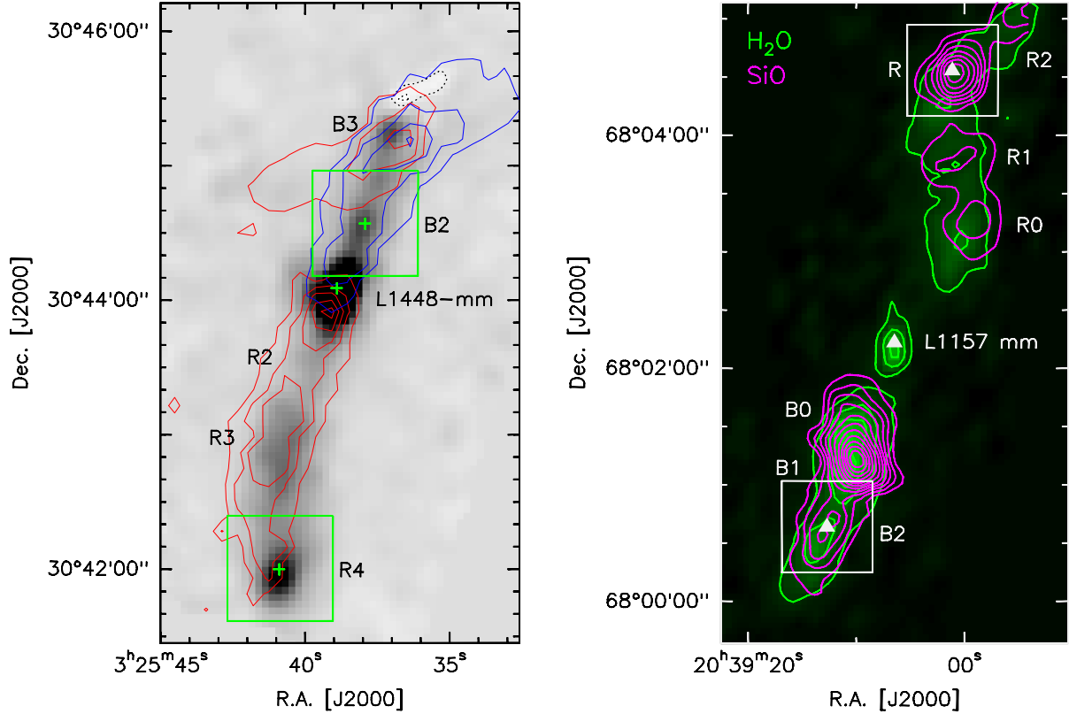
Fig. 1. PACS H 2 O 179 μm images of L1448 and L1157 (Nisini et al. 2010a, 2013). The PACS line survey positions are indicated for L1448-B2 and R4 with crosses, for L1157-B2 and R with triangles. The field of view of the PACS observations is displayed as a box at the selected positions. CO(3–2) and SiO(3–2) emissions for L1448 and L1157, respectively, are superimposed on the H 2 O maps.
