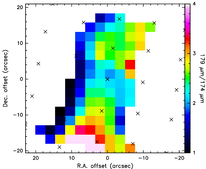
Fig. 10. Ratio between the H 2 O 2 12 -1 01 map at 179 μm and the 3 03 -2 12 map at 174 μm for L1448-B2. The ratio is shown only above a 5σ detection level in both maps. The crosses represent the pointing of the 25 spaxels.
