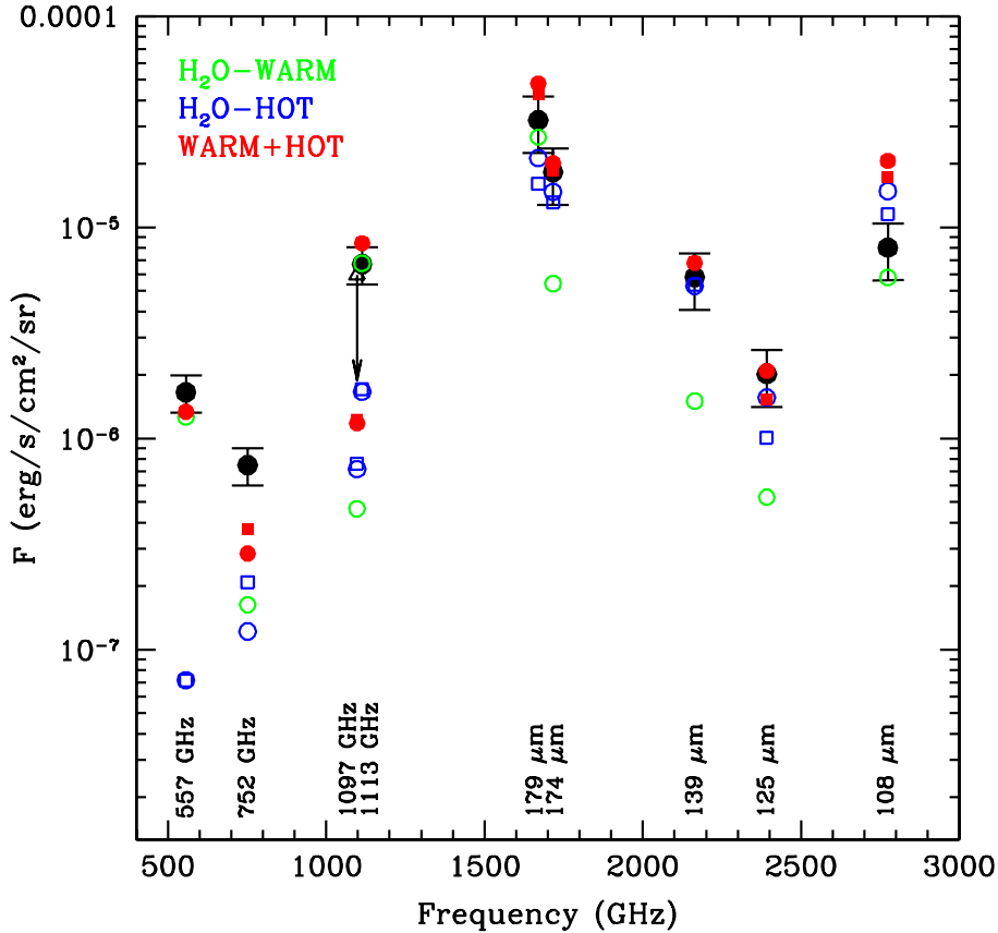
Fig. 6. Comparison between the observed \text{H}_2\text{O} fluxes (black dots) and the two best-fit models for L1448-B2, which are given in Table 2: the green model is the fit to the HIFI \text{H}_2\text{O} lines and the two blue models are the extremes of the obtained density range that fits the PACS \text{H}_2\text{O} lines (squares represent n(\text{H}_2) = 5 \times 10^5 \text{ cm}^{-3} and circles represent n(\text{H}_2) = 5 \times 10^6 \text{ cm}^{-3} ). The red model represents the sum of the fluxes predicted for each line by the green and the two blue models. The fluxes predicted by the models have been corrected for the relative predicted filling factors. Calibration uncertainties of 20% for the HIFI data and 30% for the PACS data have been assumed. The open triangle represents the upper limits of the HIFI \text{H}_2\text{O} 3_{12}-3_{03} line ( E_u = 249 \text{ K} ).
