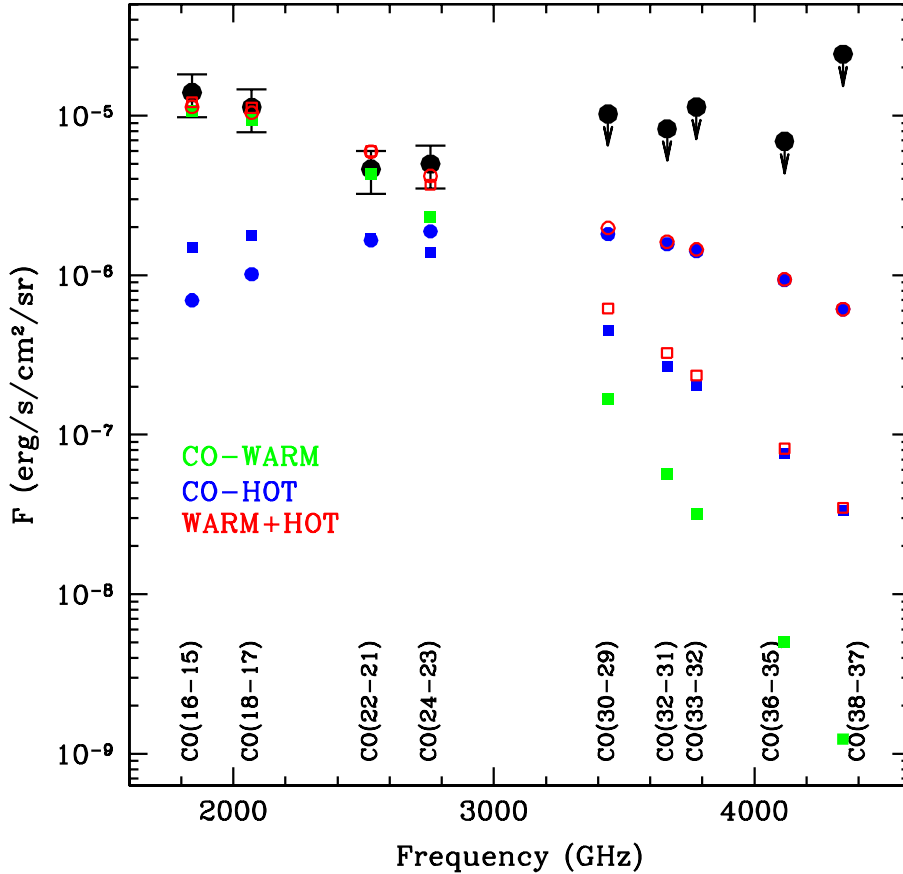
Fig. 9. Same comparison presented in Fig. 6, but for the CO fluxes measured with PACS toward L1448-B2 (both the detections and the non-detections). The two blue models represent the extremes of the density range derived from the H 2 O excitation analysis.
