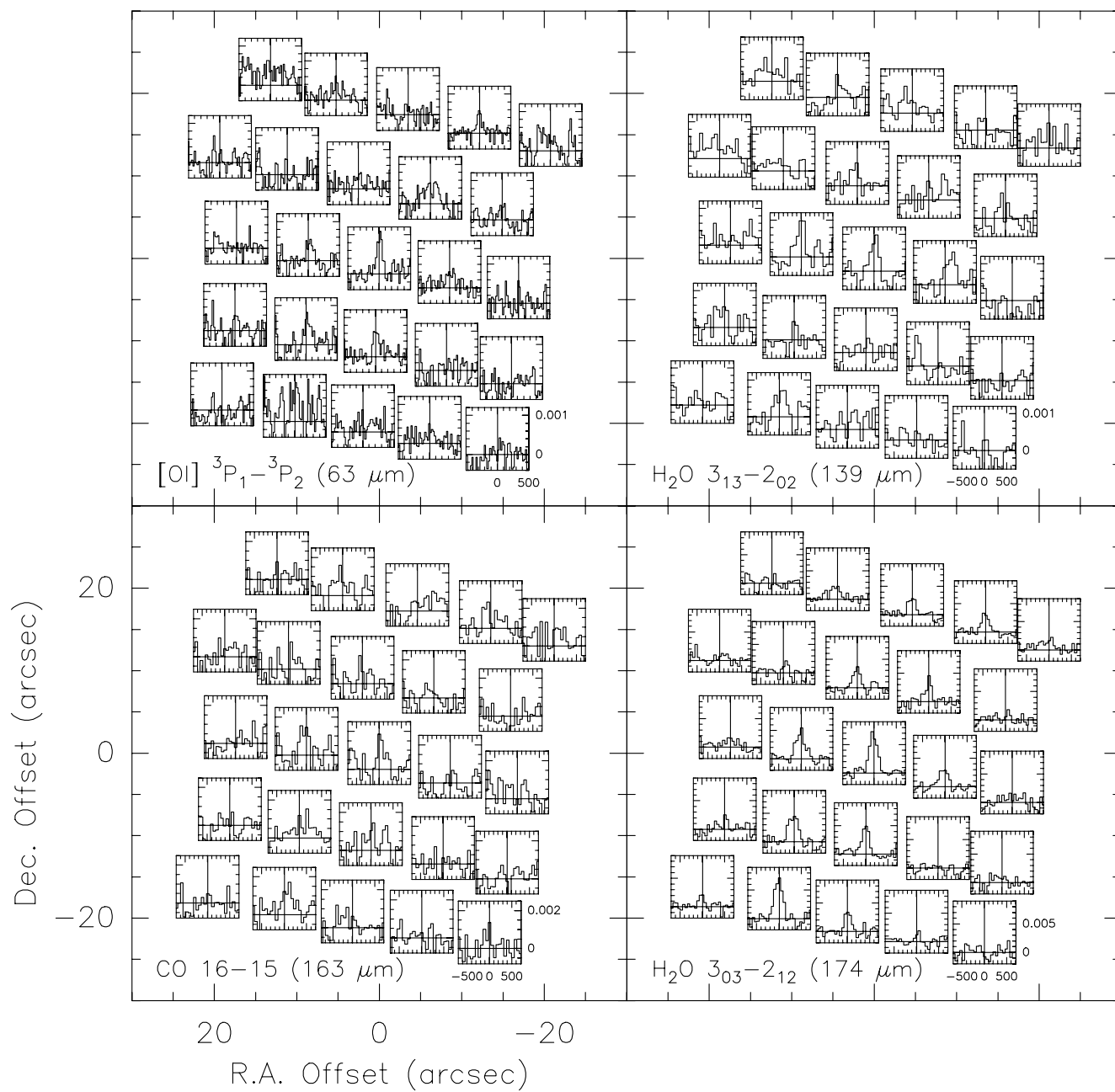
Fig. A.3. Same as Fig. A.1 for the L1157-B2 position.
