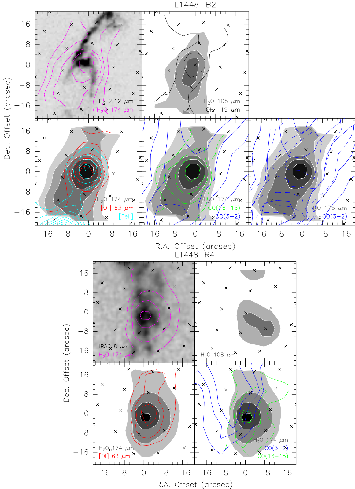
Fig. 2. Overlay between PACS H 2 O 3 03 -2 12 (174 μm), H 2 O 2 21 -1 10 (108.1 μm), [O I] 3 P 1 - 3 P 2 (63.2 μm), CO(16-15), OH (119 μm), and other tracers in the B2 (upper panel) and R4 (lower panel) shocked spots along the L1448 outflow. In particular, JCMT CO(3-2) emission (Half Power Beam Width, HPBW ~ 14'') from Nisini et al. (2013), Spitzer [Fe II] emission at 26 μm from Neufeld et al. (2009), IRAC 8 μm emission from Tobin et al. (2007), and H 2 emission at 2.12 μm from Davis & Smith (1995) are shown. In the bottom-right panel relative to L1448-B2 the EHV CO(3-2) emission ( v \gtrsim -50 km s -1 ) and the HV CO(3-2) emission ( v \lesssim -40 km s -1 ) are shown in dashed and solid lines, respectively. The contours in each map are traced every 3σ, starting from a 5σ level, except for the CO(3-2) in L1448-B2, where the contours are traced in steps of 5σ, starting from 5σ. The crosses represent the pointing of the 25 spaxels.
