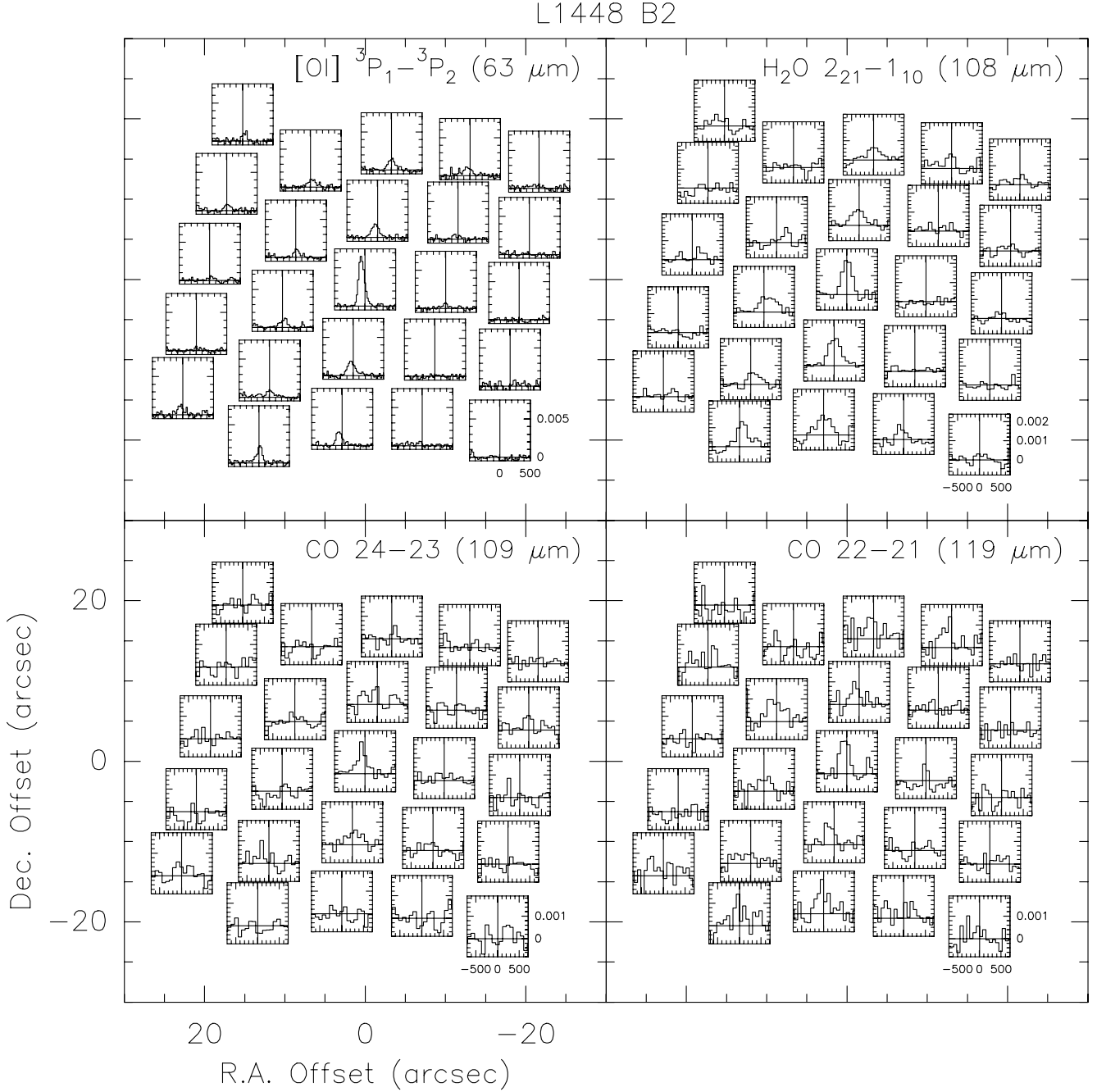
Fig. A.1. PACS spectra of the detected transitions at the L1448-B2 position. The centre of each spaxel box corresponds to its offset position with respect to the coordinates of the central shock position. The velocity ( \text{km s}^{-1} ) and intensity scale (Kelvin) are indicated for one spaxel box and refer to all spectra of the relative transition. The labels in the top-right corner of every box indicate the relative transition.
