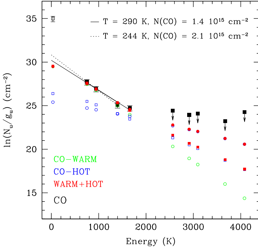
Fig. 8. Rotational diagram at L1448-B2 for the CO emission lines (both the detections and the non-detections) observed with PACS (in a 12'' beam) and the JCMT CO(3–2) line (empty symbol; beam size equal to 14'' ). Calibration uncertainties of 30% have been assumed. The solid line represents the linear fit to the four detected CO lines, the dotted line the linear fit only to the three lower excitation CO lines. As in Fig. 7, the predictions of the two best-fit models for L1448-B2 corrected for the relative predicted filling factors are shown.
