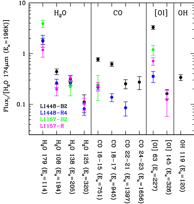
Fig. 11. Line ratios between the H 2 O, CO, [OI], and OH lines and the H 2 O 3 03 -2 12 line at 174 \mu\text{m} at all selected shock positions. 1 \sigma errors are indicated with errorbars.
