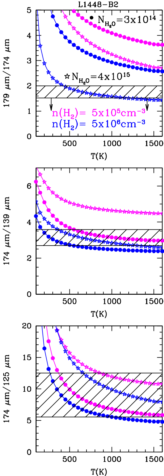
Fig. 5. Top: ratio between H 2 O 2 12 –1 01 (179 μm) and 3 03 –2 12 (174 μm) emission, as a function of T for two values of H 2 density ( n_{\text{H}_2} = 5 \times 10^5 \text{ cm}^{-3} and 5 \times 10^6 \text{ cm}^{-3} ) and two values of H 2 O column density ( N_{\text{H}_2\text{O}} = 3 \times 10^{14} and 4 \times 10^{15} \text{ cm}^{-2} ) of L1448-B2. The shaded band highlights the H 2 O ratio observed with PACS and the arrows indicate that this ratio can be considered an upper limit (see text for details). Middle and bottom: ratios between H 2 O 3 03 –2 12 (174 μm) and 3 13 –2 02 (138.5 μm) emission and between H 2 O 3 03 –2 12 (174 μm) and 4 04 –3 13 (125.4 μm) emission, respectively, as a function of T . The symbols are the same as in the top panel.
