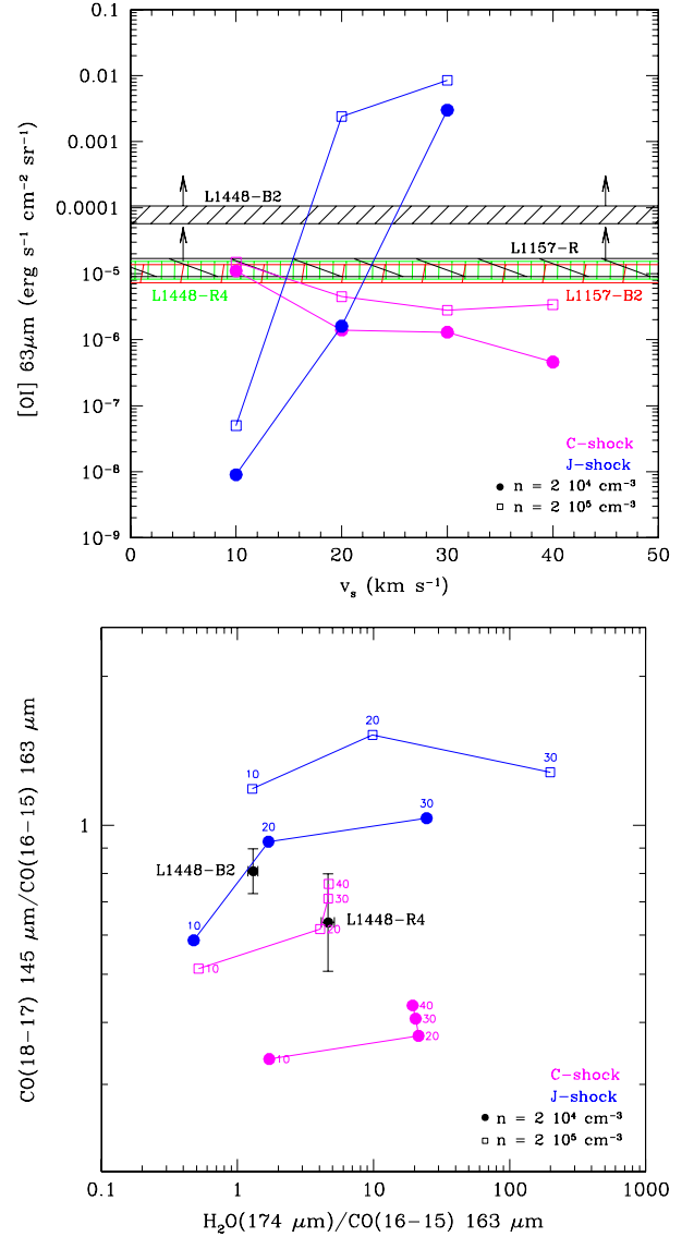
Fig. 13. Upper panel: comparison between the [OI] 3 P 1 - 3 P 2 (63.2 μm) flux observed at the investigated shock positions (shaded bands) and the corresponding theoretical values predicted by the Flower & Pineau Des Forêts (2010) shock models for C-type shocks (magenta) and J-type shocks (blue), as a function of the shock velocity in units of km s -1 . The fluxes measured in the central spaxel of the PACS maps have been used without smoothing to a common angular resolution. Calibration uncertainties of 30% have been assumed. The arrows in the plot indicate that the absolute fluxes have to be considered as lower limits; they are beam diluted because we do not resolve the emitting size of the shock. Lower panel: same comparison as in the upper panel, but for CO and H 2 O line ratios. The observed values are depicted as black dots and the errorbars represent 1σ errors. The data have been smoothed to a common angular resolution of 12''.6.
