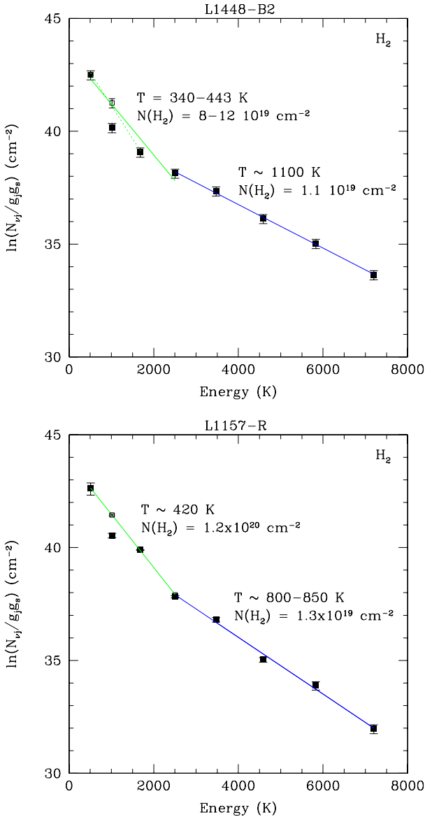
Fig. 4. Upper: rotational diagram at L1448-B2 for the H 2 emission lines detected with Spitzer by Giannini et al. (2011). The values have been derived from the H 2 fluxes integrated over a 13'' area for comparison with the PACS data. The black dots are the observed values, whereas the empty dot represents the H 2 S(1) line corrected for an ortho-to-para ratio equal to 1 (see Giannini et al. 2011). The green solid line represents the linear fit to the S(0)–S(3) H 2 lines, while the green dotted line is the fit obtained using the S(0)–S(2) H 2 lines. Finally, the blue line is the linear fit to the S(3)–S(7) lines. The resulting parameters ( T, N ) or range of parameters of the linear fits are reported in the diagram. Lower: H 2 rotational diagram at L1157-R. The symbols are the same as in the upper panel.
