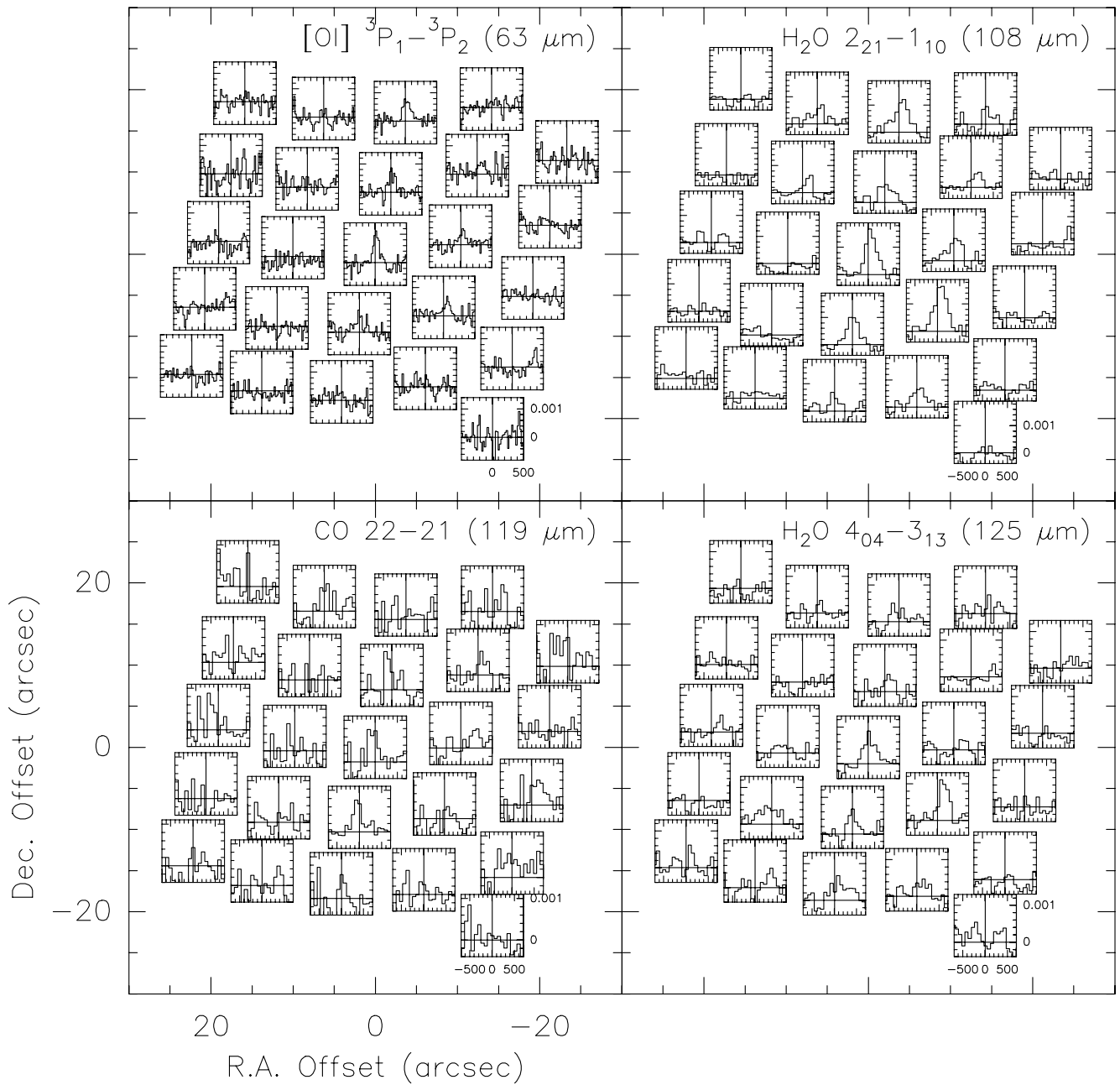
Fig. A.2. Same as Fig. A.1 for the L1448-R4 position.
