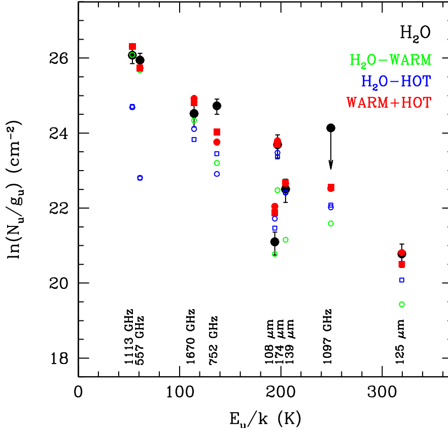
Fig. 7. H 2 O rotational diagram at L1448-B2. Calibration uncertainties of 20% for the HIFI data and 30% for the PACS data have been assumed. The predictions of the two best-fit models for L1448-B2, corrected for the relative predicted filling factors, are shown (see Table 2 and Fig. 6). Symbols are as in Fig. 6.
