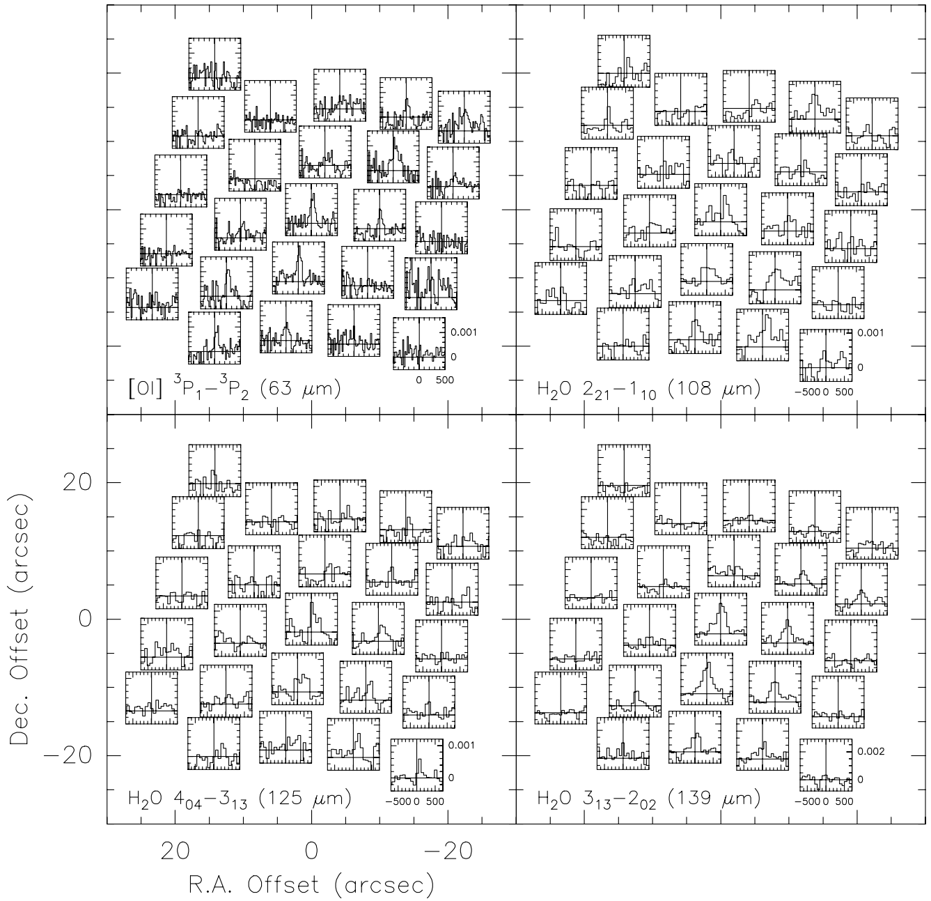
Fig. A.4. Same as Fig. A.1 for the L1157-R position.
