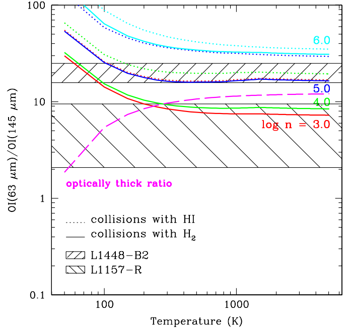
Fig. 12. Optically thin [OI]63 \mu\text{m} /[OI]145 \mu\text{m} flux ratios as a function of temperature are shown in dotted lines for collisions with atomic hydrogen H and in solid lines for collisions with molecular hydrogen H 2 (as in Liseau et al. 2006). The logarithms of the density (in cm -3 ) are indicated for each curve. The broken line outlines the ratio of optically thick lines. Observed line ratios are depicted by the shaded areas for the L1448-B2 position and the L1157-R position. The data have been smoothed to a common angular resolution of 12''6.
