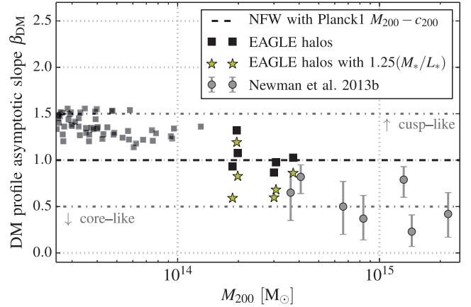
Figure 4. The asymptotic logarithmic slope of the inner DM density profile, \beta_{\text{DM}} , as a function of halo mass, M_{200} . The dashed line shows the NFW value of -1 . The large black squares show the values measured for the six massive clusters in our EAGLE sample and the small black squares those measured for smaller EAGLE clusters. The yellow stars show the slopes that would be inferred for our sample if the stellar mass-to-light ratio is overestimated by 25 per cent (see Section 5.3 for details). The grey circles with error bars are the values inferred by Newman et al. (2013b). As in Fig. 3, the grey dash-dotted lines demarcate slopes that may be construed as ‘core-like’ and ‘cuspy’.
