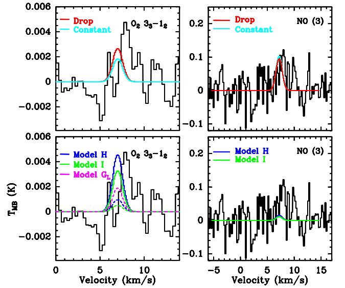
Fig. 8. Best-fit model spectra produced by different abundance profiles for O 2 3 3 -1 2 and NO (3) are overlapped over the observed spectra. In the bottom figures, solid fit spectra show H 0 and I 0 models and dashed fit spectra show models H L , I L , and G L . For NO, Case 2 is adopted.
