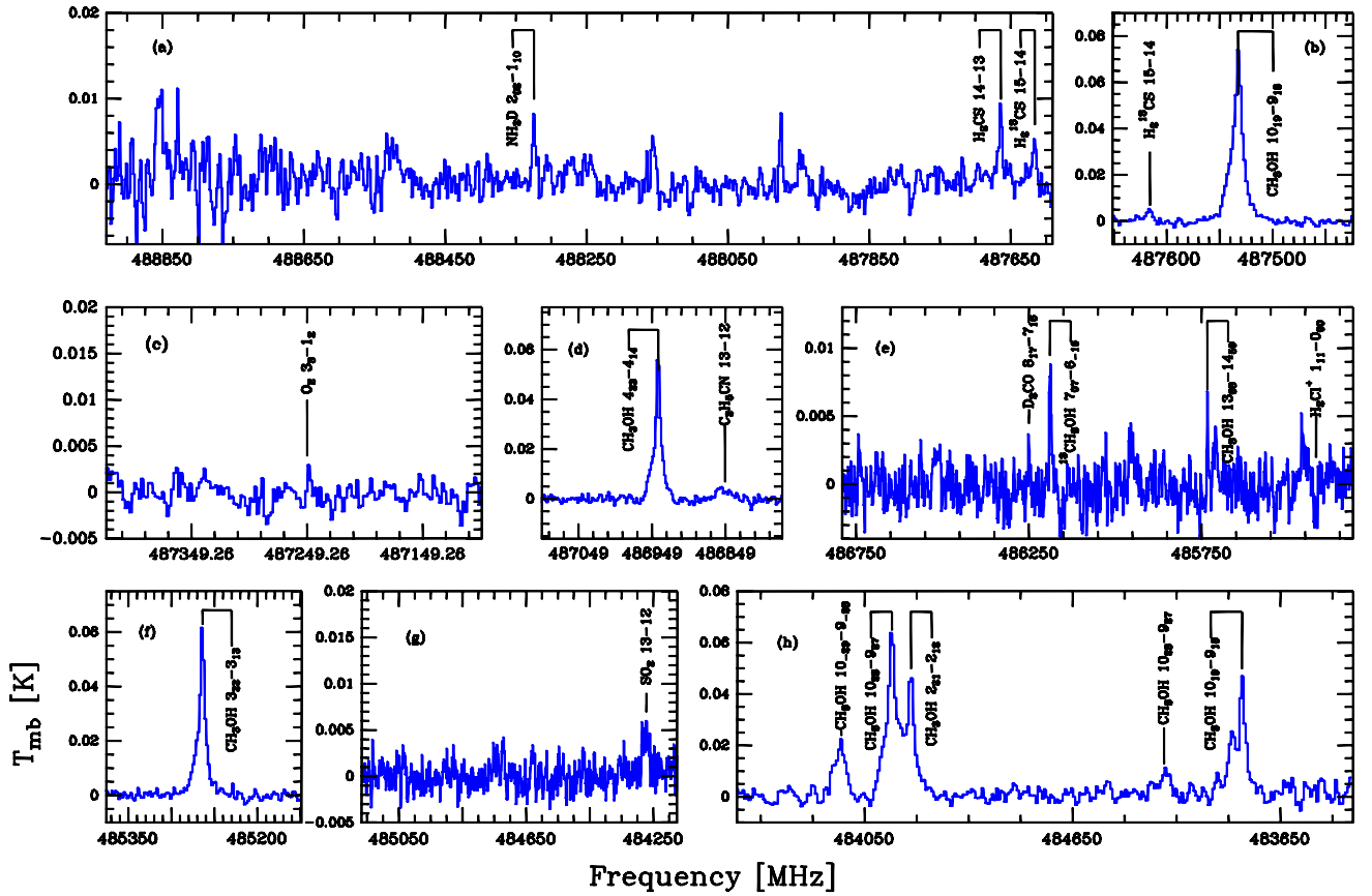
Fig. A.1. Spectrum of Fig. 2 magnified over certain velocity ranges. In panel c) the O 2 3 3 -1 2 transition is shown. Identifications refer to the 7.0 km s -1 component.
