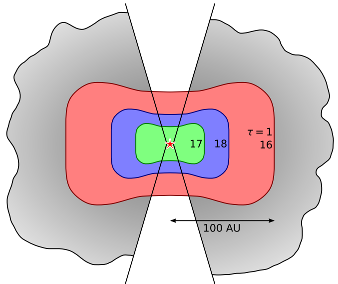
Figure 3. Illustration of the hot core ( T > 100 \text{ K} ) in IRAS2A. The red and blue areas show the \tau_\nu = 1 surfaces for the 3_{12-3_{03}} lines of \text{H}_2^{16}\text{O} and \text{H}_2^{18}\text{O} , with a difference in area that explains the different intensities observed with Herschel -HIFI (Figure 1). The green area shows the maximum size of the \text{H}_2^{17}\text{O} \tau_\nu = 1 surface allowed by the 3\sigma upper limit from HIFI. The red area is the same as that of the spatially resolved \text{H}_2^{18}\text{O} 3_{13-2_{20}} emission detected with the PdBI (Persson et al. 2012). The hot core is embedded inside a colder envelope ( T < 100 \text{ K} ; shaded gray), extending out to 10^4 \text{ AU} (not drawn to scale).
