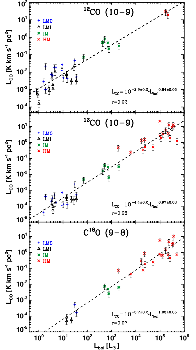
Fig. 6. Line luminosity of the ^{12}\text{CO} J = 10-9 (top), ^{13}\text{CO} J = 10-9 (middle) and \text{C}^{18}\text{O} J = 9-8 (bottom) spectra for low-mass Class 0 (LM0; blue pluses), low-mass Class I (LMI; black triangles), intermediate-mass (IM; green asterisks) and high-mass (HM; red crosses) YSOs versus their bolometric luminosity. The black dashed line represents the linear function that fits the logarithm of the plotted quantities.
