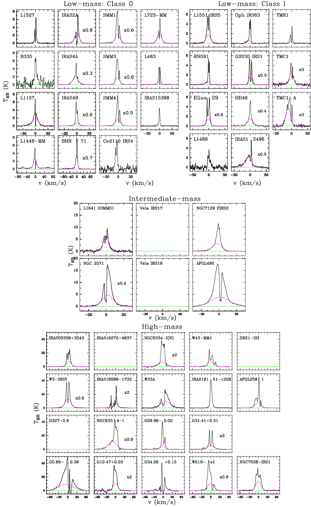
Fig. B.4. ^{12}\text{CO } J=3-2 spectra for low-, intermediate and high-mass YSOs, observed with the JCMT. The green line represents the baseline level and the pink Gaussian profile the broad velocity component for those sources for which a two Gaussian decomposition has been performed. All the spectra have been shifted to zero velocity. The numbers indicate where the spectra have been scaled for greater visibility.
