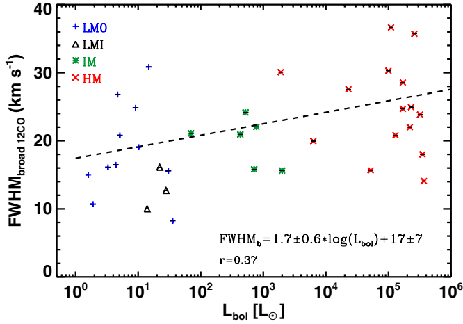
Fig. 4. FWHM of the broad velocity component identified in the ^{12}\text{CO } J = 10-9 line profiles for each type of YSOs versus their bolometric luminosities. Low-mass Class 0 (LM0) sources are indicated with blue pluses, low-mass Class I (LMI) with black triangles, intermediate-mass (IM) YSOs with green asterisks and high-mass (HM) objects with red crosses. For the high-mass sources, the ^{12}\text{CO } J = 3-2 width is used instead. The black dashed line indicates the linear function that fits the relation between the FWHM and the logarithm of L_{\text{bol}} .
