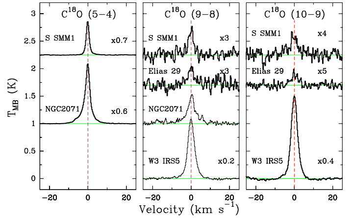
Fig. 3. Same as Fig. 2 but for the \text{C}^{18}\text{O} spectra from the observed transitions: J = 5-4 ( left ), J = 9-8 ( centre ) and J = 10-9 ( right ). For details about these objects see Appendix A.
