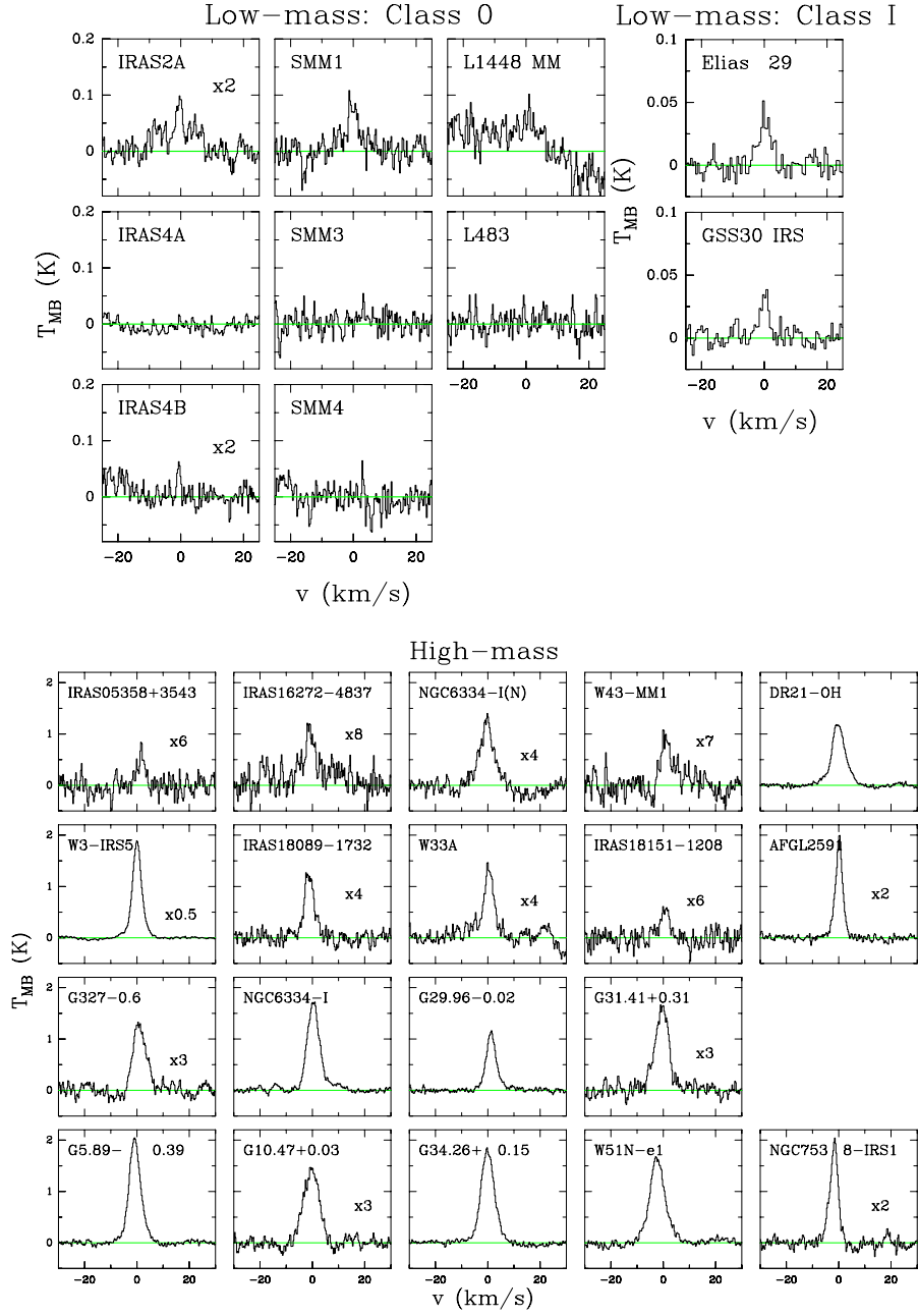
Fig. A.5. Same as Fig. A.1 but for the \text{C}^{18}\text{O } J = 10-9 spectra of the observed low- and high-mass YSOs. In the case of the high-mass sources, the YSOs are organised as in Fig. A.2. The line wings of the 3_{12}-3_{03} water transition for the high-mass sources have been fitted with a Gaussian profile, subtracted, and the residuals plotted to isolate the \text{C}^{18}\text{O } J = 10-9 emission line.
