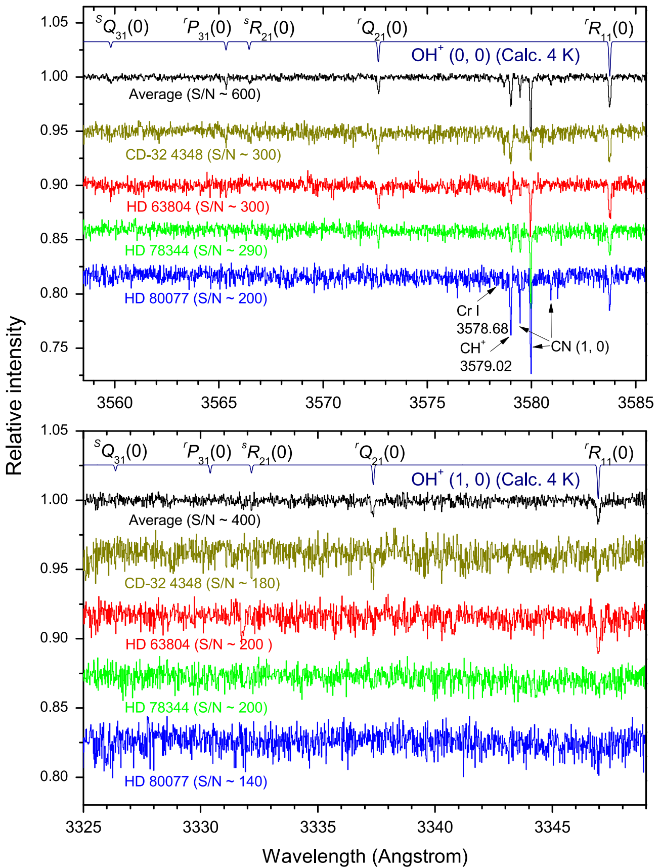
Figure 2. Spectra of the \text{OH}^+ A^3\Pi-X^3\Sigma^- (0, 0) and (1, 0) bands. From top to bottom in each panel: calculated 4 K spectrum, averaged spectrum, and individual spectra toward four high reddened stars. Spectra of the observed targets are normalized to pseudo-continuum, i.e., all broad features including stellar lines are eliminated for clarity. The narrow interstellar lines of \text{CH}^+ , \text{Cr I} , and \text{CN} are marked in the upper panel. The overall S/N estimated from the displayed wavelength regions are also presented for each spectrum.
