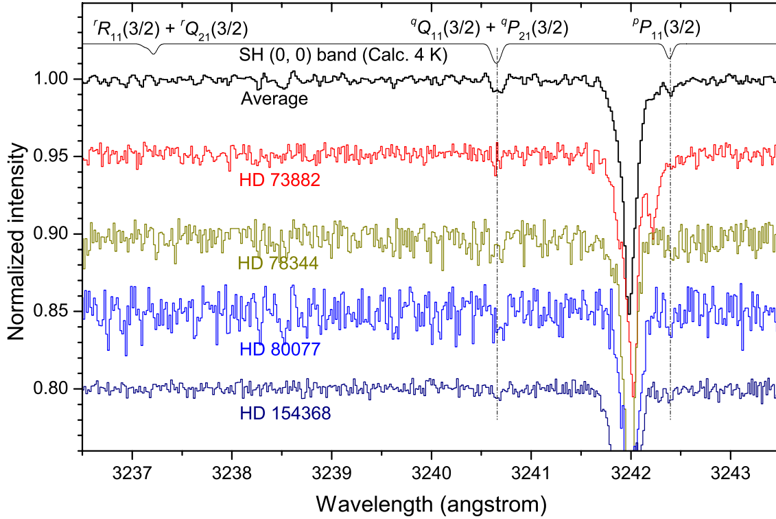
Fig. 1. Spectra of the SH A^2\Sigma^+ - X^2\Pi (0, 0) band. From top to bottom: calculated 4 K spectrum, averaged spectrum, and individual sight line spectra toward HD 73882, HD 78344, HD 80077, and HD 154368. Spectra of the observed targets are normalized to pseudo-continuum, i.e., all broad features including stellar lines are eliminated for clarity. The wavelength scale of each spectrum has been shifted so that interstellar absorption lines appear at rest wavelengths.
