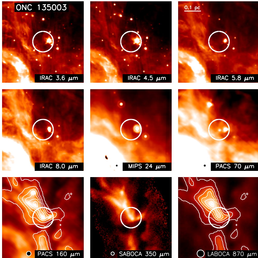
Figure A1. Multi-wavelength images of the additional PBR source 135003. This source is located in the OMC 2/3 region where there are high levels of nebosity. The source immediately west of 135003 is HOPS 59, a Class I protostar. Notice that 135003 resides at an inflection point of the filament traced at longer wavelengths. The white circle marks the location of 135003 and is 30'' in radius. The black circles at the bottom are the respective beam sizes. The contours overlaid on the 160 \mu\text{m} and 870 \mu\text{m} images are the 870 \mu\text{m} emission contours at [0.5, 1.0, 1.5, 2.0, 2.5, and 3.0] Jy beam ^{-1} .
