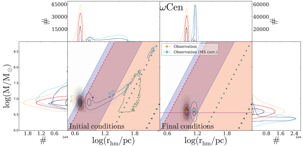
Figure 13. The same as Fig. 6, but for the cluster \omega Cen.
