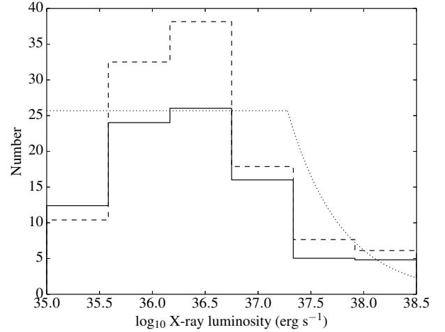
Fig. 10. X-ray luminosity distributions of the present-day population of LMXBs, including UCXBs, with neutron star accretors in the Galactic Bulge. The star formation history width is \sigma = 0.5 \text{ Gyr} (solid line) and \sigma = 2.5 \text{ Gyr} (dashed line). These distributions include hydrogen-rich as well as hydrogen-poor LMXBs, and both persistent sources and transient sources in outburst. The dotted line shows the X-ray luminosity function parametrized by Gilfanov (2004, sample “All” in Table 3) using the best-fitting normalization of K_1 = 440.4 , and further adjusted for the bin width of our histograms to allow for direct comparison.
