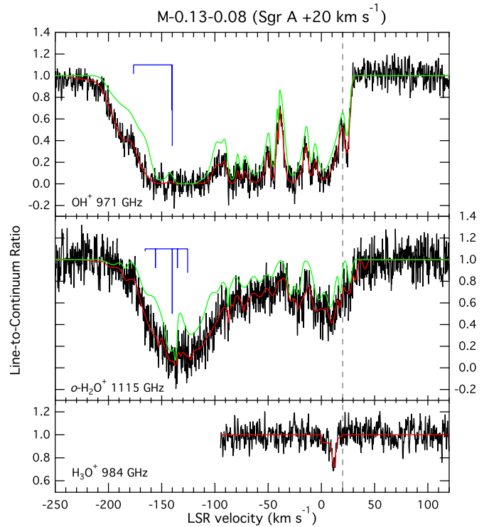
Figure 2. Single sideband normalized spectra toward M-0.13-0.08 (Sgr A +20 km s -1 cloud) showing transitions of \text{OH}^+ , \text{H}_2\text{O}^+ , and \text{H}_3\text{O}^+ . Stick diagrams above spectra show the hyperfine structure where applicable. Red curves are fits to the absorption features, and green curves show only the strongest hyperfine component of the fits. The vertical dashed line marks the systemic velocity of the background source. Vertical axes give line-to-continuum ratio, with labels alternating between the left and right sides for clarity.
