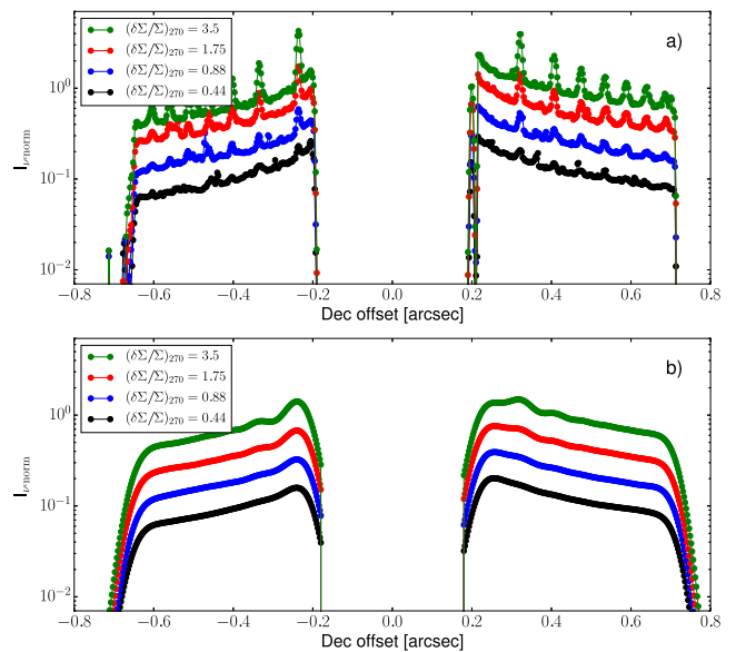
Figure 5. Cross-section of the calculated images with different surface density perturbations at original resolution, as calculated by RADM3D (Panel a), and after convolved with a 0.06 arcsec circular Gaussian PSF (Panel b).
