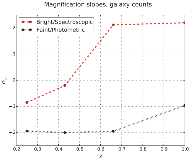
Figure 1. The number counts magnification slopes ( \alpha_s ) for a bright ( 18 < i_{AB} < 22.5 ) and faint ( 22.5 < i_{AB} < 24.1 ) from the COSMOS sample. Values are extrapolated outside of this redshift range.
