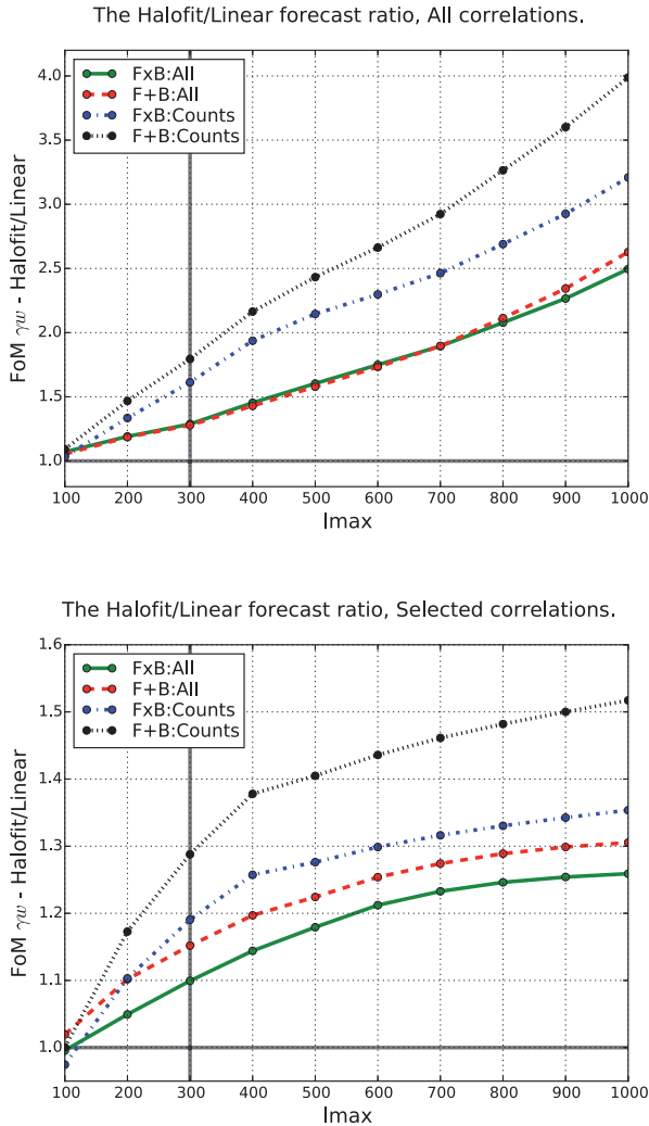
Figure A1. Forecast ratio between including the Halofit contributions and only the linear (Eisenstein & Hu 1998, EH) power spectrum. The figure of merit is \text{FoM}_{\gamma w} and the lines correspond to \text{F}\times\text{B}:\text{All} , \text{F}+\text{B}:\text{All} , \text{F}\times\text{B}:\text{Counts} and \text{F}+\text{B}:\text{Counts} . In the top/bottom panel, the ratios include/exclude correlations entering into non-linear scales ( k > k_{\text{max}} ). A vertical line at l_{\text{max}} = 300 marks the fiducial value.
