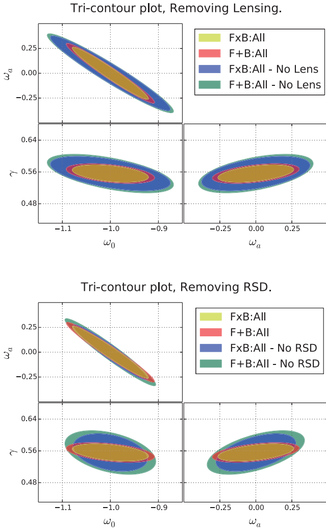
Figure B2. Contour plots of w_0 , w_a and \gamma . The three sub-plots show the Fisher matrix 1\sigma contours, marginalizing over the DETF parameters and galaxy bias. In the upper plot, two ellipses are the fiducial F×B:All and F+B:All, while two remove WL observables. The bottom plot similarly shows the fiducial F×B:All and F+B:All, and then two contours in real space.
