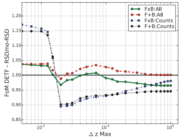
Figure 10. FoM ratio between redshift and real space when varying the largest redshift separations in the cross-correlations ( \Delta Z_{\text{Max}} ). In the two plots corresponding to \text{FoM}_\gamma and \text{FoM}_{\text{DETF}} , the four lines are the probes \text{F}\times\text{B:All} , \text{F+B:All} , \text{F}\times\text{B:Counts} and \text{F+B:Counts} .
