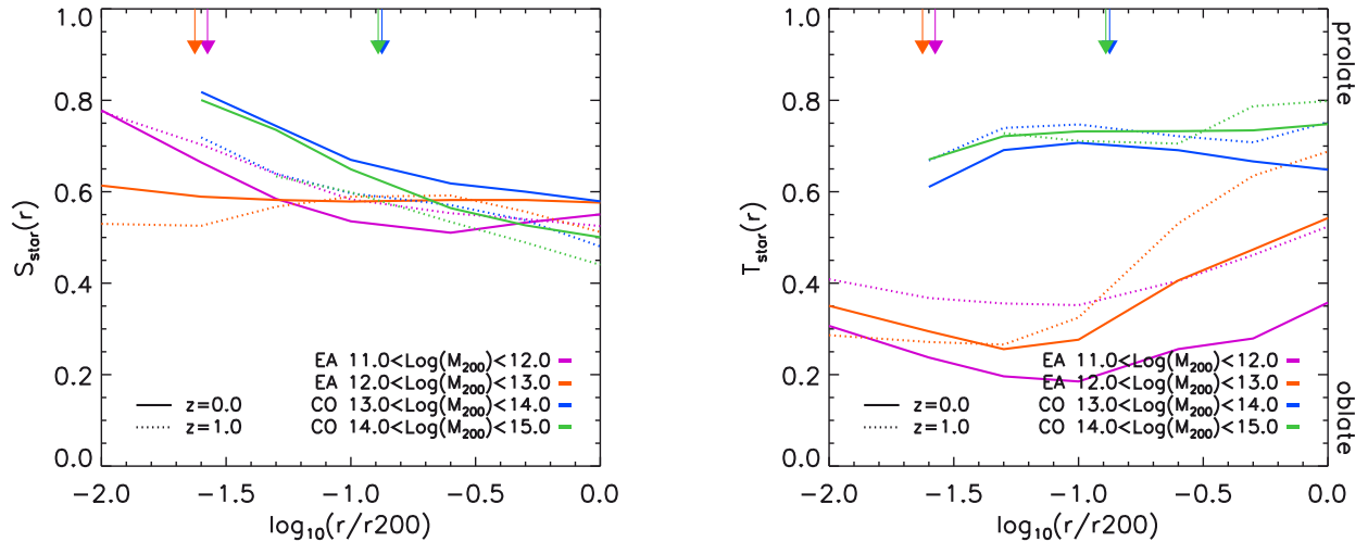
Figure 6. Stellar shape parameters (sphericity on the left, triaxiality on the right) as a function of distance from the centre of the halo for haloes in different halo mass bins (see legend). Distances have been rescaled to the mean halo radius in each mass bin, r_{200}^{\text{crit}} to ease the comparison of the results for different masses. Different colours indicate different simulations, whereas different line styles refer to different redshifts. The distribution becomes less spherical and more prolate with increasing distance from the halo centre. Vertical arrows indicate the median values of the half-mass radii in stars, r_{\text{half}}^{\text{star}} , which can be considered a proxy for the typical extent of a galaxy. The blue arrow lies beneath the green one.
