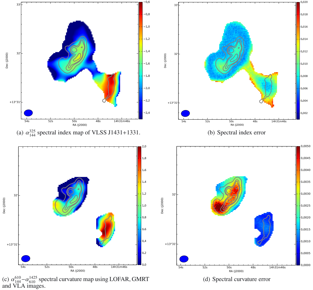
Fig. 3. In all panels 1425 MHz high resolution VLA contours overlaid (levels as in Fig. 2). The beam size is indicated in the lower left corner.
