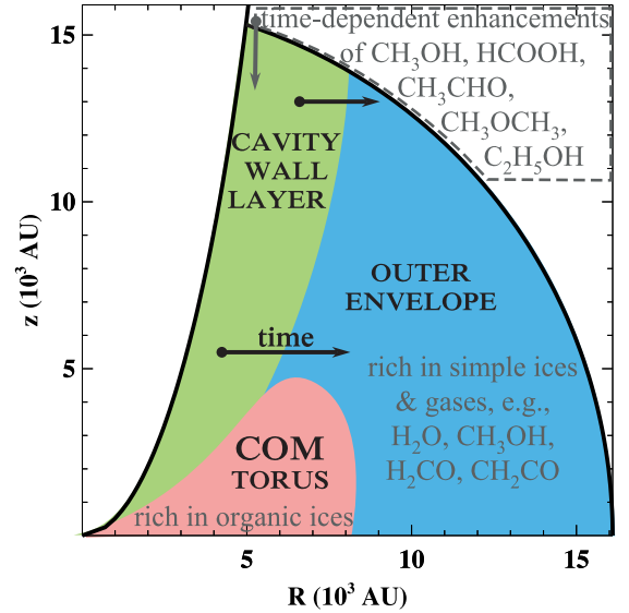
Figure 10. An illustration summarizing the key zones of the envelope-cavity system and the major species and their phases therein. The motion of the cavity wall layer with time is indicated with two arrows. COM stands for complex organic molecules.
