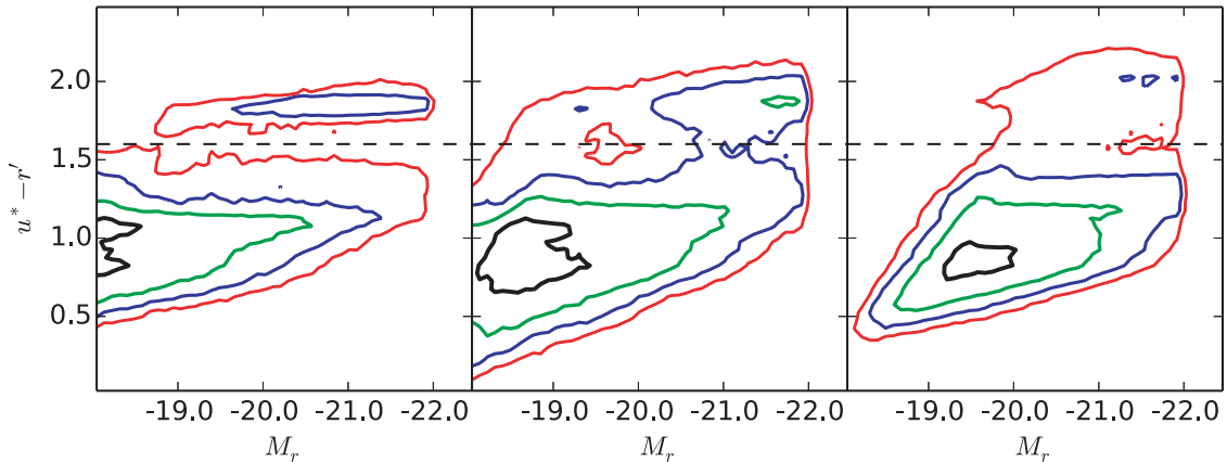
Figure 1. Colour–magnitude diagrams for CFHTLenS galaxies for three redshift bins 0.2 \leq z_p < 0.4 , 0.4 \leq z_p < 0.6 , 0.6 \leq z_p < 0.8 from left to right. The contours show density of galaxies in colour–magnitude space relative to the peak density in that redshift bin. The colour is rest-frame u_{\text{CFHT}}^* - r_{\text{CFHT}}' , the horizontal dashed line shows the colour 1.6 used to separate red and blue populations.
