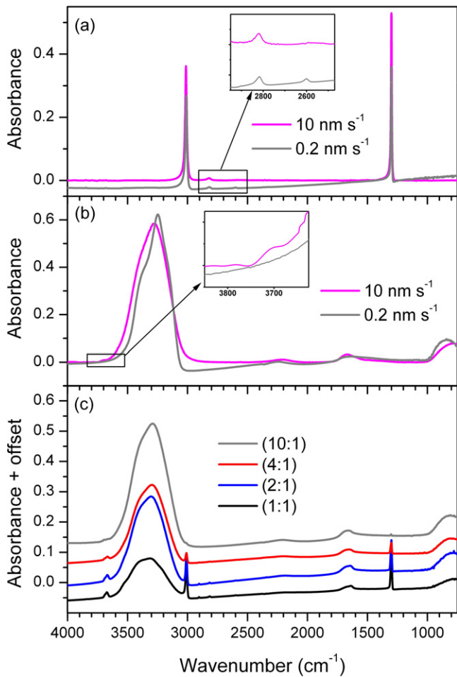
Figure 2. Mid-infrared spectra of (a) pure and compact CH 4 ice grown at 30 K (0.4 \mu\text{m} , front deposition) using two different deposition rates, (b) pure and compact H 2 O ice grown at 30 K (0.6 \mu\text{m} , front deposition) with two different deposition rates, and (c) porous H 2 O:CH 4 ice mixtures grown at 30 K (0.4 \mu\text{m} , background deposition) with a 0.2 nm s -1 deposition rate.
