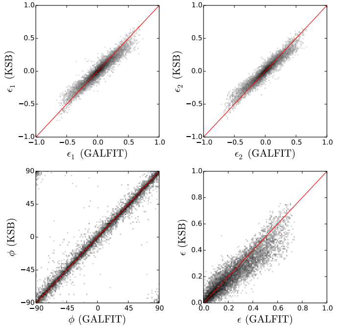
Fig. 6. Comparison of shape measurements from KSB and GALFIT. Grey scales show the number of points per bin in logarithmic scale. Red lines show y = x . Top : ellipticity components in Cartesian coordinates. Bottom left : position angles, \phi , in degrees. The periodicity of \phi (of 180 deg) can be seen in the top left and bottom right corners of the plot. Bottom right : galaxy ellipticities.
