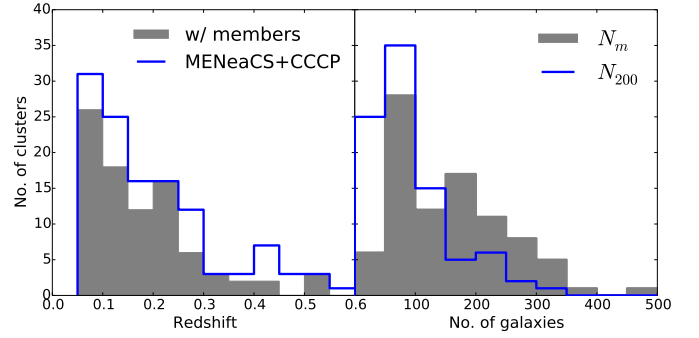
Fig. 1. Left: redshift distributions of all MENeACS+CCCP clusters (blue histogram) and clusters used in this study (gray filled histogram). Right: distributions of number of spectroscopic members, N_m (gray filled histogram), and number of spectroscopic members within r_{200} , N_{200} (blue histogram). Abell 2142, with N_m = 1052 and N_{200} = 731 , is not shown.
