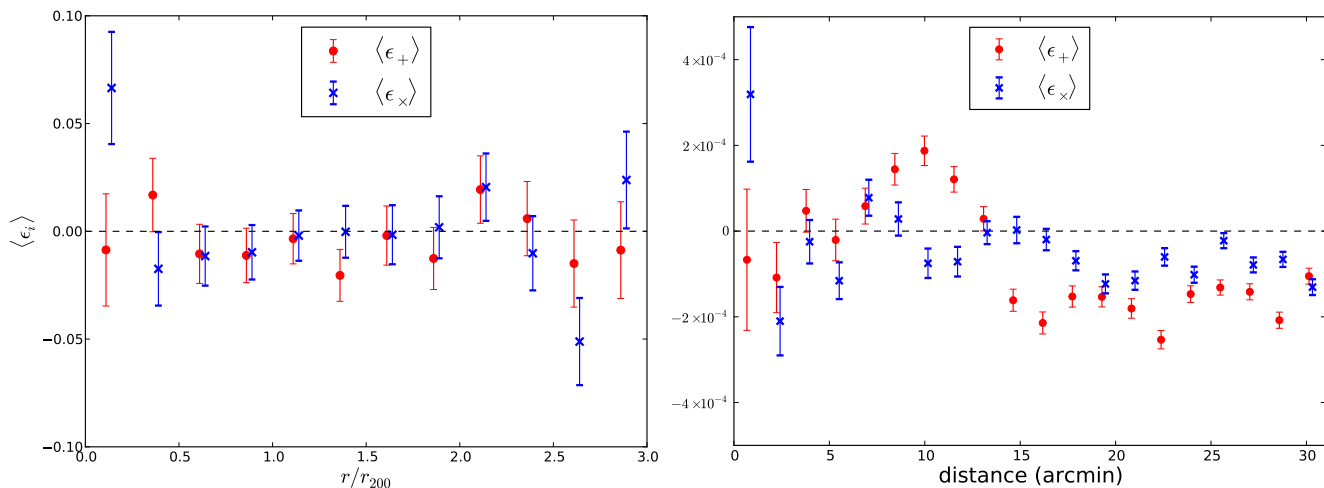
Fig. 7. Alignment signal from control samples measured with KSB, with data points shifted horizontally for clarity. Left: 3666 foreground galaxies in the direction of 73 clusters as a function of distance from the cluster, in units of r_{200} . Right: stars in the magnitude range 17 < m_r < 22 as a function of angular distance from the center of each cluster. Typically, r_{200} \sim 10' . Note the different vertical scales in each plot.
