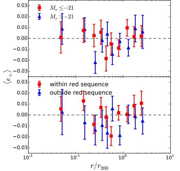
Fig. 10. Average alignment \langle \epsilon_+ \rangle from KSB for spectroscopically confirmed members divided by galaxy properties: by rest-frame r -band absolute magnitude ( top ), and color with respect to each cluster’s red sequence ( bottom ).
