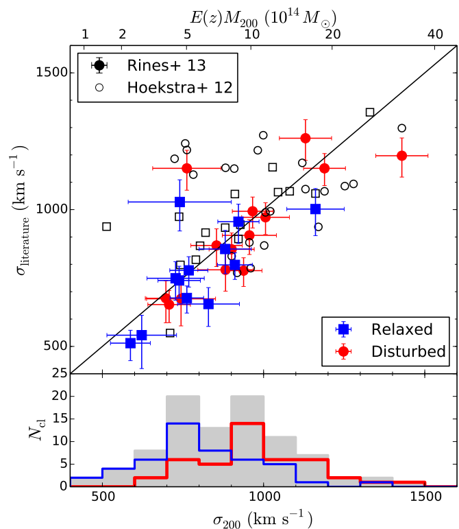
Fig. 3. Top : comparison between velocity dispersions calculated from spectroscopic members in this work with those in Rines et al. (2013) , and with velocity dispersions calculated by fitting a single isothermal sphere to the weak lensing profile ( Hoekstra et al. 2012 ) for CCCP clusters used in this work. Errorbars are not shown for the latter for clarity. Squares and circles show relaxed and disturbed clusters, respectively. The black line shows the one-to-one relation, and the top axis shows E(z)M_{200} for a given \sigma_{200} from the Evrard et al. (2008) relation. Bottom : distribution of velocity dispersions of the full sample. The gray histogram shows the total distribution, with the blue and red histograms showing the distributions for relaxed and disturbed clusters, respectively.
