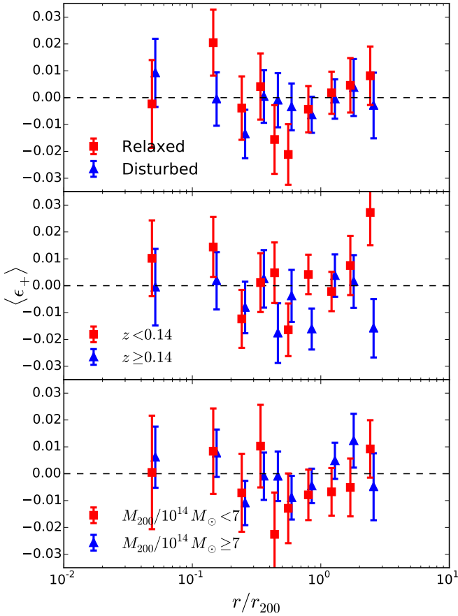
Fig. 9. Average alignment \langle \epsilon_+ \rangle from KSB for spectroscopically confirmed members, divided by cluster properties: by dynamical state ( top ; see Sect. 3.1.1), redshift ( middle ), and dynamical mass ( bottom ). The latter two thresholds are the median values of the cluster sample.
