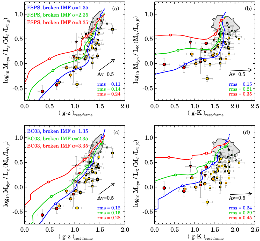
Figure 7. M/L vs. rest-frame color for an IMF with different slopes between 1 M_{\odot} and 4 M_{\odot} . Below 1 M_{\odot} and above 4 M_{\odot} , this IMF has a Salpeter slope, as defined according to Equation (5). We use FSPS (top row) and BC03 (bottom row) models with solar metallicity ( Z = 0.02 ). Based on the rms scatter, the models favor an IMF with a slope of \alpha = 1.35 over \alpha = 2.35 . The FSPS model with a broken IMF of \alpha = 1.35 is able to reproduce both the M/L vs. g - z and g - K rest-frame color.
