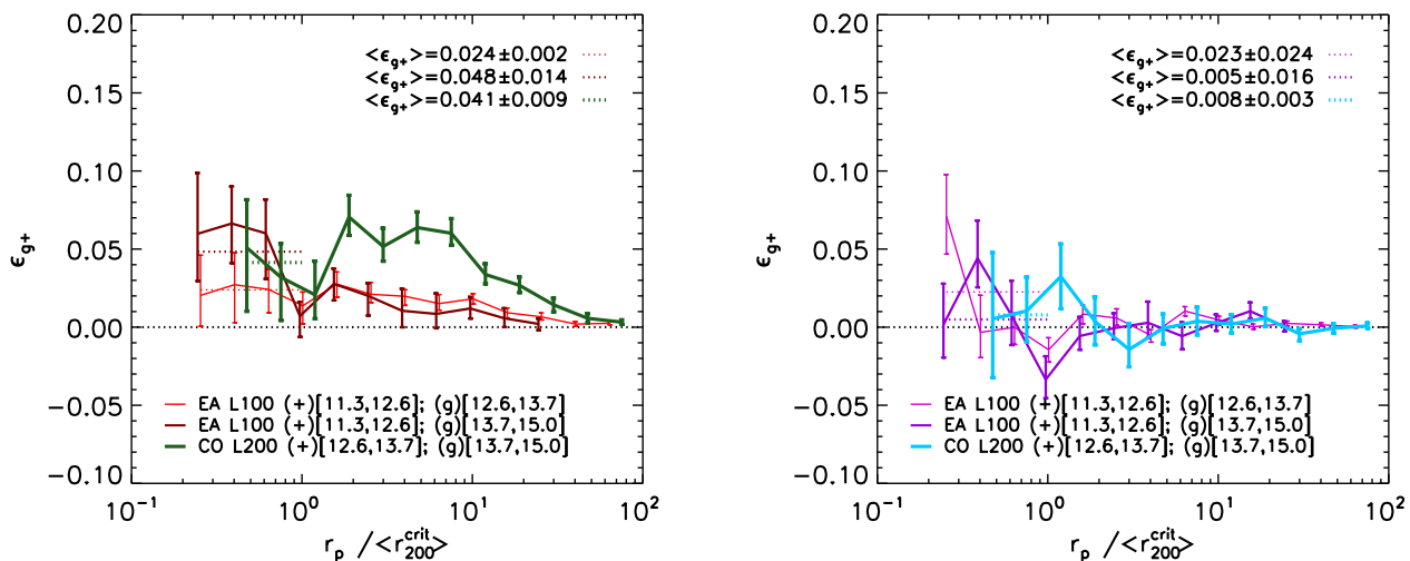
Figure 8. Values of the observationally accessible proxy for orientation–direction alignment, \epsilon_{g+} (see equation 9), as a function of the projected separation r_p . Only pairs that are separated by less than 2.5 h^{-1} Mpc along the projected axis are considered for this analysis. The error bars indicate one sigma bootstrap errors. In the left-hand panel, the orientation of the subhalo is measured using all the stellar particles whereas in the right-hand panel, only stars within the r_{\text{half}}^{\text{star}} are used, which greatly reduces the alignment. Thicker lines indicate higher masses. The coloured dotted lines show the average value of \epsilon_{g+} within the virial radius of the central galaxy. Observational measurements from Sifón et al. (2015) constrained the average ellipticity to be \epsilon_{g+} = -0.0037 \pm 0.0027 .
