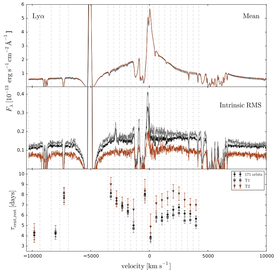
Figure 6. Velocity-binned results for the \text{Ly}\alpha \lambda 1215 emission line. The top and middle panels show the mean and intrinsic rms ( \sigma_0 ) spectra, respectively. The bottom panel shows the centroid of the cross-correlation function for each individual velocity bin, corrected to the rest frame of NGC 5548. Velocity bins with no lag measurement contain too little total flux to reliably characterize the variations. In each case, the black line represents the entire dataset, and the T1 (first 85 visits) and T2 (last 86 visits) subsets are shown in gray and orange, respectively. The large gap at around -5000 \text{km s}^{-1} avoids the region of the spectrum affected by geocoronal emission and Galactic absorption.
