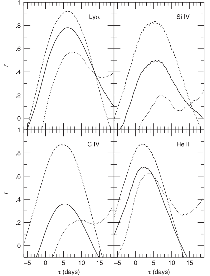
Figure 4. Interpolated cross-correlation functions (ICCFs) computed by cross-correlating each emission-line light curve with the 1367 Å continuum light curve. The solid line is the ICCF for the entire data set. The dashed line is for the T1 subsample (the first 85 visits) and the dotted line is for the T2 subsample (the last 86 visits).
