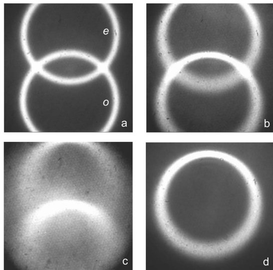
FIG. 3. SPDC emission patterns observed with an intensified CCD at 6 cm from a 1-mm-thick BBO, for three focusing conditions of the pump beam: (a) plane wave ( \sigma = 0.86 \pm 0.07 mrad), (b) intermediate ( \sigma = 12.0 \pm 0.5 mrad), and (c) extreme ( \sigma = 32 \pm 1 mrad) with exposure times of 1, 1.3, and 0.8 s, respectively. In each of these pictures, the upper and lower rings correspond to extraordinary ( e ) and ordinary ( o ) photons, respectively. Picture (d) was taken behind a polarizer to highlight the ordinary ring in (b). All four images cover a space angle of 220 \times 220 mrad 2 and contain 100 accumulated snapshots.
