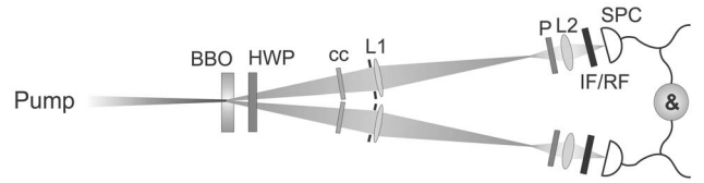
FIG. 2. Schematic view of the experimental setup (see text for details).
