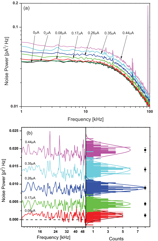
FIG. 2. (Color online) Example of the noise power data analysis. (a) Noise-power spectra for a Pt atomic chain of \sim 3 atoms in length having a conductance G = 1.52 (2e^2/h) and a Fano factor F = 0.192 . The peaks are due to spurious signals that could not be fully shielded. (b) Same data after subtracting the thermal noise and correcting for the roll-off. The spurious signals are effectively removed by the subtraction procedure.
