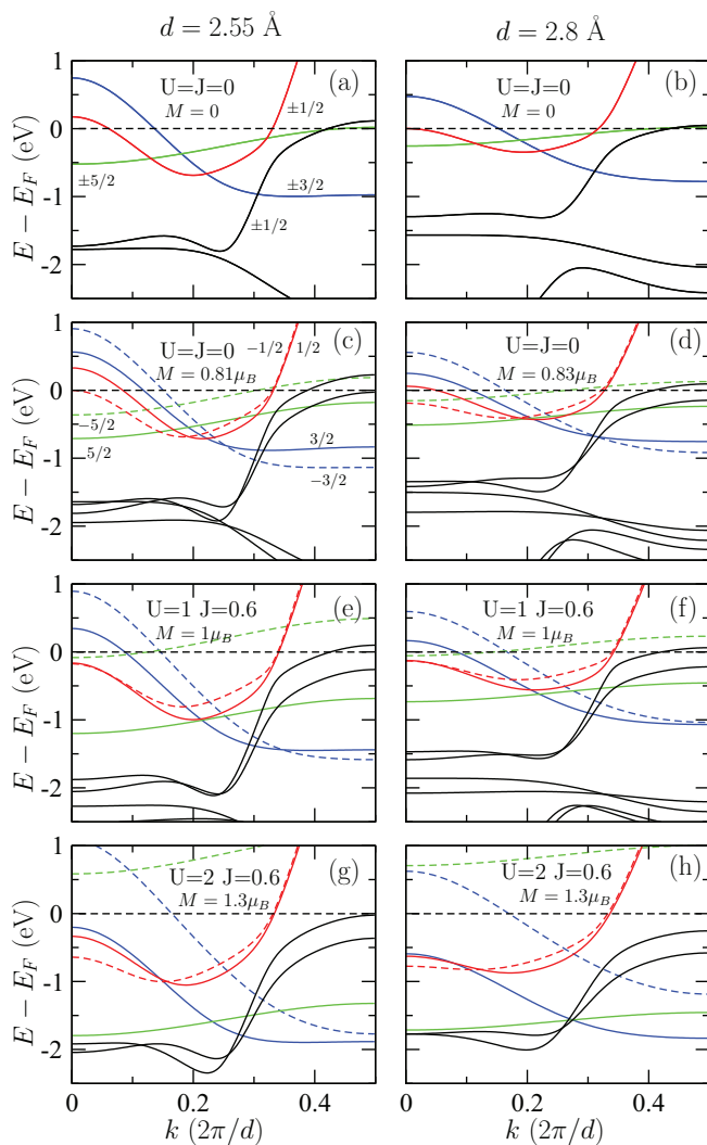
FIG. 5. (Color online) Tight-binding relativistic band structures of infinite Pt chains at interatomic spacings of d = 2.55 Å (low strain, shown in the left column) and 2.80 Å (large strain, right column). (a)–(d) for U = J = 0 ; (e) and (f) for U = 1 eV and J = 0.6 eV; (g) and (h) for U = 2 eV and J = 0.6 eV. For U = J = 0 , the bands of nonspin polarized calculation are shown in (a) and (b). A magnetic state with the spin moment M parallel to the chain axis (c) and (d) is lower in energy than a nonmagnetic one in all cases. Local interactions introduced via U and J only enhance magnetism further. The various bands important for magnetism and conductance are drawn with different colors (see text) and are labeled by half-integer total angular momentum m_j (along the chain axis) in the upper panels (a)–(d). Spin-polarized bands for magnetic solutions with positive (negative) m_j are displayed as full (broken) curves.
