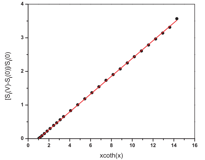
FIG. 3. (Color online) Reduced excess noise Y = [S_I(V) - S_I(0)]/S_I(0) for a Pt atomic chain. The excess noise is given as a function of X = x \coth(x) = (eV/2k_B T) \coth(eV/2k_B T) , for a chain having a conductance of G = 1.425 \pm 0.01(2e^2/h) at a length of about two atoms in the chain.
