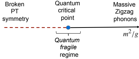
FIG. 1: (Color online) Zero-temperatures phase diagram of Reggeon quantum chain. For large harmonic potential (to the right of the plot), the chain exhibits a massive Zigzag mode and exponentially decaying correlations \langle \phi_\ell \phi_m \rangle \sim e^{-|x_\ell - x_j|/m} . In the regime around the quantum critical point (blue dot), the chain is quantum fragile with long-ranged, power-law correlations among transverse vibrations \langle \phi_\ell \phi_m \rangle \sim \frac{1}{|x_\ell - x_j|^{2-\eta_A^*}} with \eta_A^* computed in Eq. (19).
