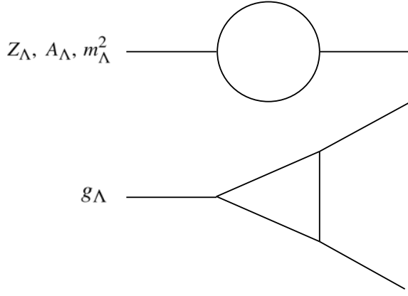
FIG. 3: Feynman diagrams for the flow equations to capture quantum fluctuations of the transverse vibrations in the chain. The straight line denotes the Zigzag propagator and the crossing of three lines the cubic interaction vertex.
