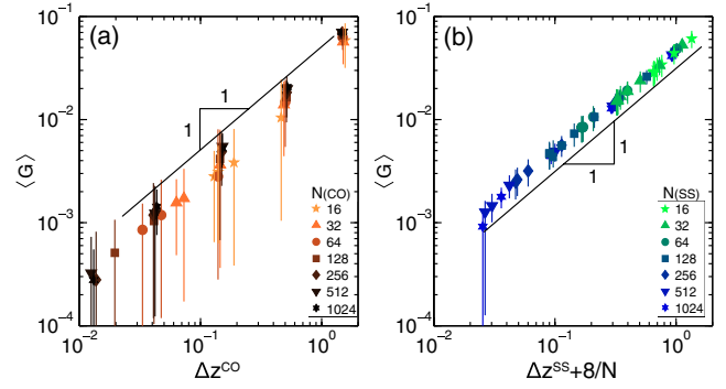
FIG. 5 (color online). (a) Linear scaling of \langle G \rangle with \Delta z^{\text{CO}} for CO packings. The error bars indicate the RMS fluctuations in G . (b) Linear scaling of \langle G \rangle with \Delta z^{\text{SS}} + 8/N for SS packings—where \Delta z^{\text{SS}} := z - z_{\text{iso}}^{\text{SS}} = z - 4 .
